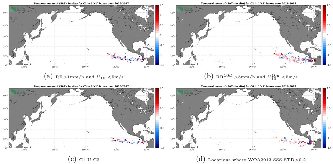
Figure 11: Temporal mean gridded over spatial boxes of size 1^\circ \times 1^\circ of \Delta SSS (SMAP-L2-RSS-V3-70KM - Surface drifters) for 4 different subdatasets corresponding to: RR > 1\text{mm/h} and U_{10} < 5\text{m/s} (a), RR^{10d} > 5\text{mm/h} and U_{10}^{10d} < 5\text{m/s} (b), C1 U C2 (c), Locations where WOA2013 SSS STD > 0.2 (d).
