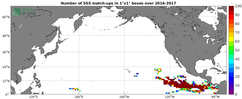
Figure 3: Number of SSS match-ups between Surface drifters SSS and the SMAP-L2-RSS-V3-70KM SSS product for the North Pacific Ocean Pi-MEP region over 1^\circ \times 1^\circ boxes and for the full satellite product period.
