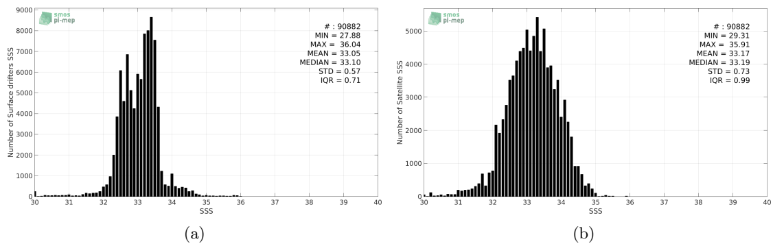
Figure 2: Histograms of SSS from Surface drifters (a) and SMAP-L2-RSS-V3-70KM (b) considering all match-up pairs per bins of 0.1 over the North Pacific Ocean Pi-MEP region and for the full satellite product period.
