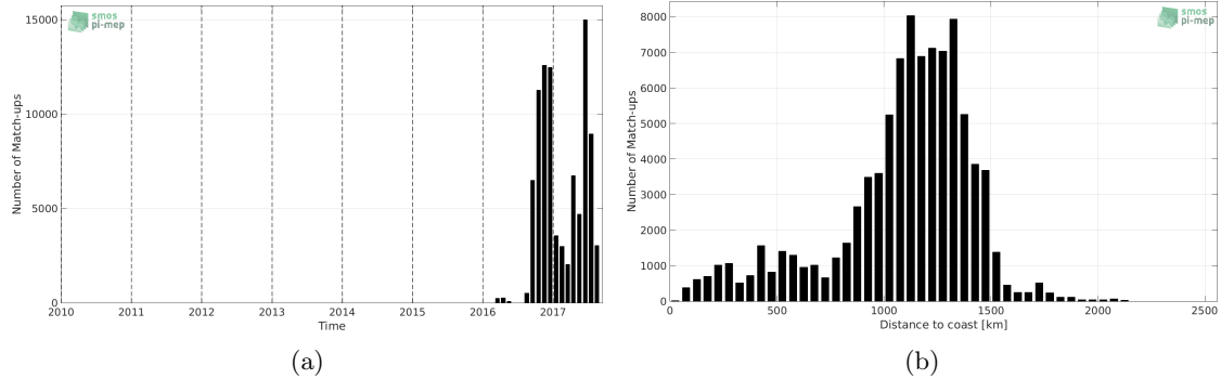
Figure 1: Number of match-ups between Surface drifters and SMAP-L2-RSS-V3-70KM SSS as a function of time (a) and as function of the distance to coast (b) over the North Pacific Ocean Pi-MEP region and for the full satellite product period.
