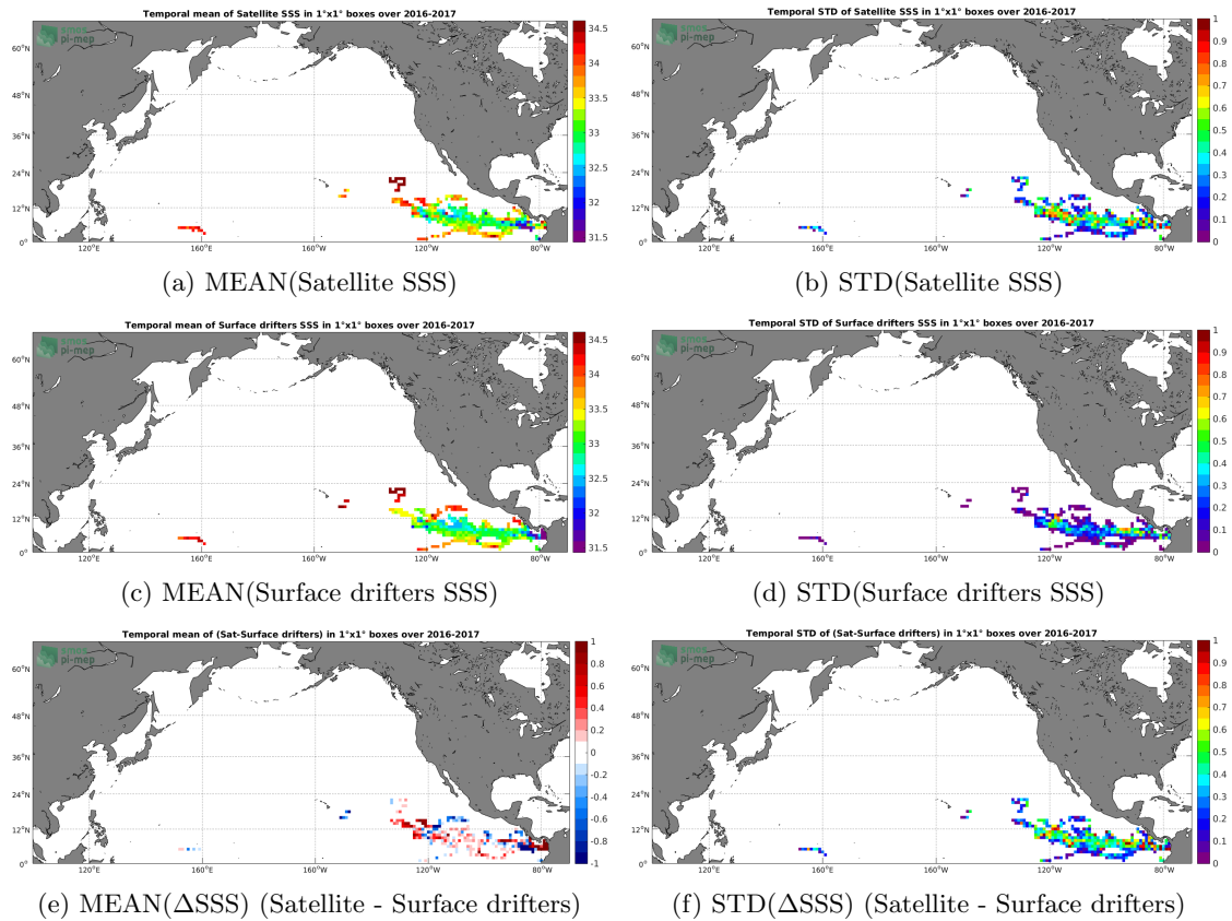
Figure 5: Temporal mean (left) and STD (right) of SSS from SMAP-L2-RSS-V3-70KM (top), Surface drifters (middle), and of \Delta SSS (Satellite - Surface drifters). Only match-up pairs are used to generate these maps.
