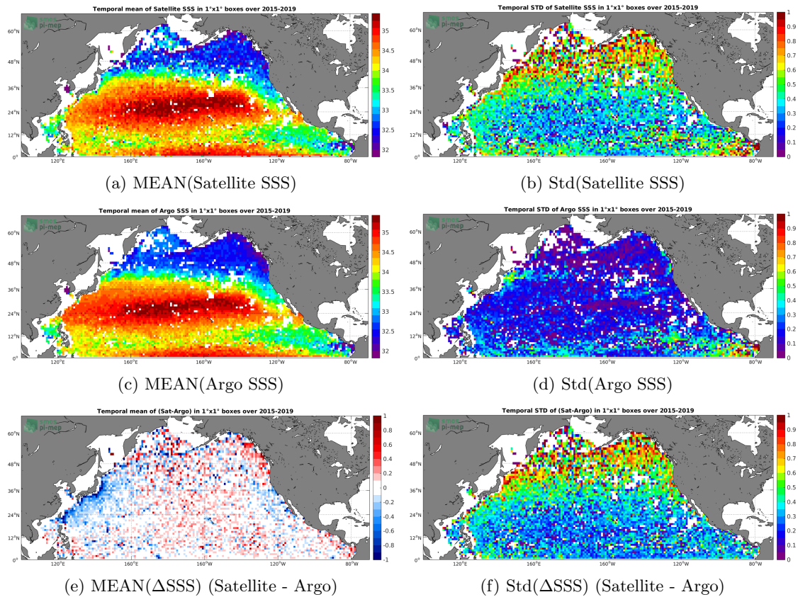
Figure 6: Temporal mean (left) and Std (right) of SSS from SMAP-L2-RSS-V3-70KM (top), Argo (middle), and of \Delta SSS (Satellite - Argo). Only match-up pairs are used to generate these maps.
