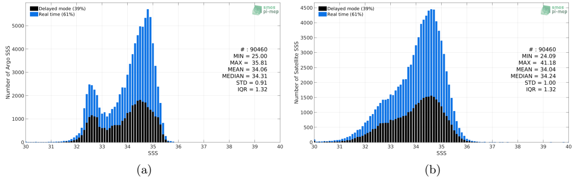
Figure 2: Histograms of SSS from Argo (a) and SMAP-L2-RSS-V3-70KM (b) considering all match-up pairs per bins of 0.1 over the North Pacific Ocean Pi-MEP region and for the full satellite product period.
