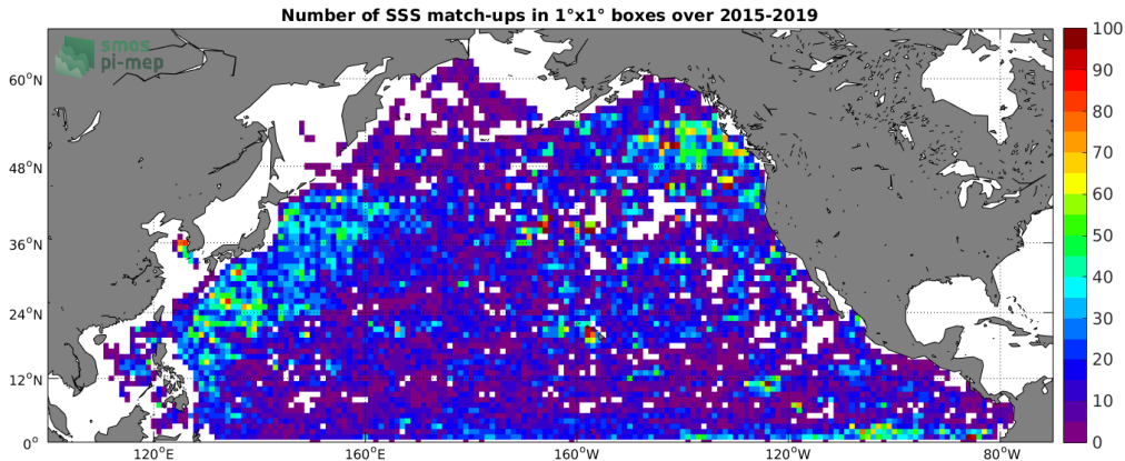
Figure 4: Number of SSS match-ups between Argo SSS and the SMAP-L2-RSS-V3-70KM SSS product for the North Pacific Ocean Pi-MEP region over 1°x1° boxes and for the full satellite product period.
