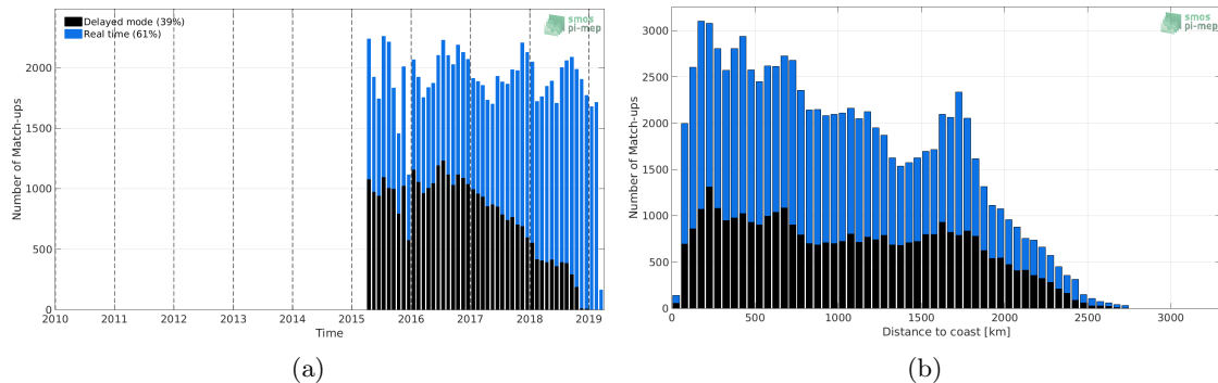
Figure 1: Number of match-ups between Argo and SMAP-L2-RSS-V3-70KM SSS as a function of time (a) and as function of the distance to coast (b) over the North Pacific Ocean Pi-MEP region and for the full satellite product period.
