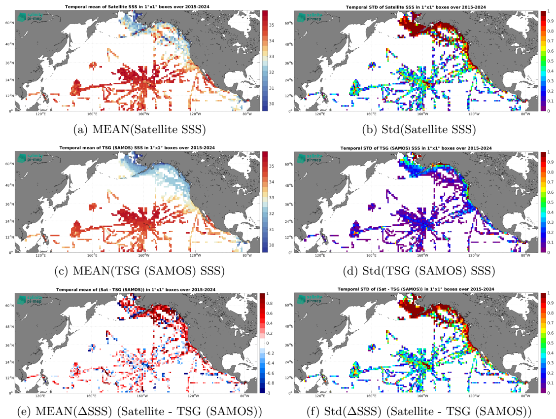
Figure 7: Temporal mean (left) and Std (right) of SSS from SMAP SSS L2 v5.0 (JPL) (top), TSG (SAMOS) (middle), and of \Delta SSS (Satellite - TSG (SAMOS)). Only match-up pairs are used to generate these maps.
