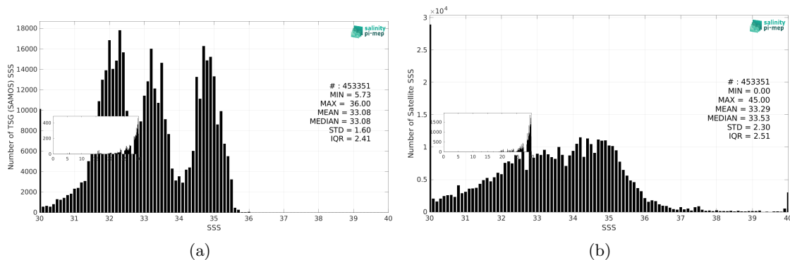
Figure 3: Histograms of SSS from TSG (SAMOS) (a) and SMAP SSS L2 v5.0 (JPL) (b) considering all match-up pairs per bins of 0.1 over the North Pacific Ocean Pi-MEP region and for the full satellite product period.
