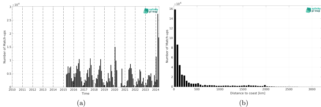
Figure 2: Number of match-ups between TSG (SAMOS) and SMAP SSS L2 v5.0 (JPL) SSS as a function of time (a) and as function of the distance to coast (b) over the North Pacific Ocean Pi-MEP region and for the full satellite product period.
