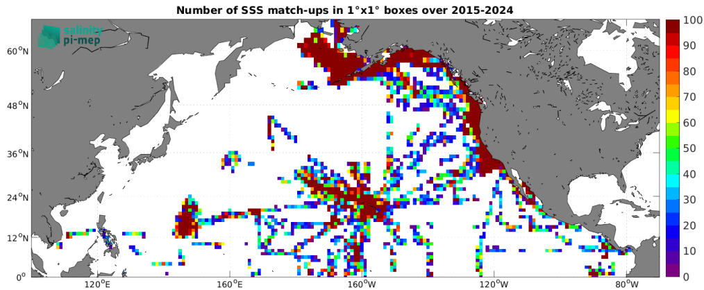
Figure 5: Number of SSS match-ups between TSG (SAMOS) SSS and the SMAP SSS L2 v5.0 (JPL) SSS product for the North Pacific Ocean Pi-MEP region over 1^\circ \times 1^\circ boxes and for the full satellite product period.
