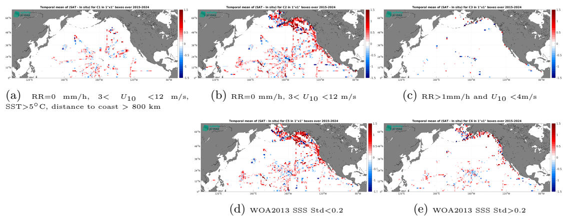
Figure 14: Temporal mean gridded over spatial boxes of size 1^\circ \times 1^\circ of \Delta SSS (SMAP SSS L2 v5.0 (JPL) - TSG (SAMOS)) for 5 different subdatasets corresponding to:RR=0 mm/h, 3 < U_{10} < 12 m/s, SST>5°C, distance to coast > 800 km (a), RR=0 mm/h, 3 < U_{10} < 12 m/s (b), RR>1mm/h and U_{10} < 4 m/s (c), WOA2013 SSS Std<0.2 (d), WOA2013 SSS Std>0.2 (e).
