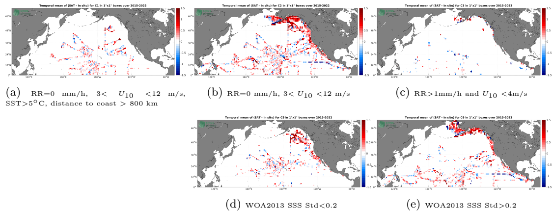
Figure 12: Temporal mean gridded over spatial boxes of size 1^\circ \times 1^\circ of \Delta\text{SSS} (SMAP SSS L2 v5.0 (JPL) - TSG (SAMOS)) for 5 different subdatasets corresponding to:RR=0 mm/h, 3 < U_{10} < 12 m/s, SST >5^\circ\text{C} , distance to coast > 800 km (a), RR=0 mm/h, 3 < U_{10} < 12 m/s (b), RR >1 mm/h and U_{10} < 4 m/s (c), WOA2013 SSS Std <0.2 (d), WOA2013 SSS Std >0.2 (e).
