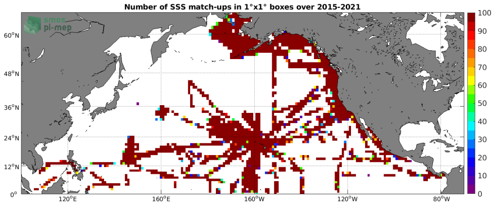
Figure 4: Number of SSS match-ups between TSG (SAMOS) SSS and the SMAP SSS L2 v5.0 (JPL) SSS product for the North Pacific Ocean Pi-MEP region over 1°x1° boxes and for the full satellite product period.
