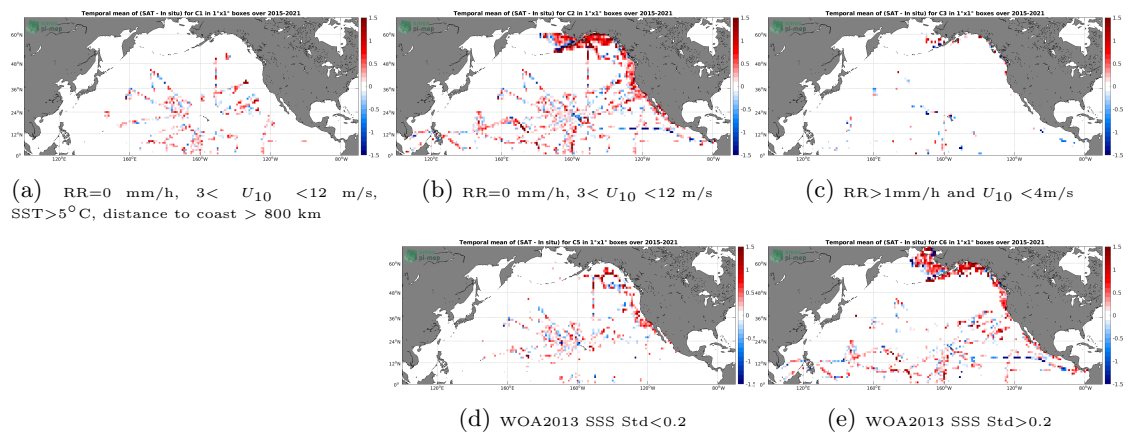
Figure 12: Temporal mean gridded over spatial boxes of size 1°x1° of \Delta SSS (SMAP SSS L2 v5.0 (JPL) - TSG (SAMOS)) for 5 different subdatasets corresponding to:RR=0 mm/h, 3 < U_{10} < 12 m/s, SST>5°C, distance to coast > 800 km (a), RR=0 mm/h, 3 < U_{10} < 12 m/s (b), RR>1mm/h and U_{10} < 4 m/s (c), WOA2013 SSS Std<0.2 (d), WOA2013 SSS Std>0.2 (e).
