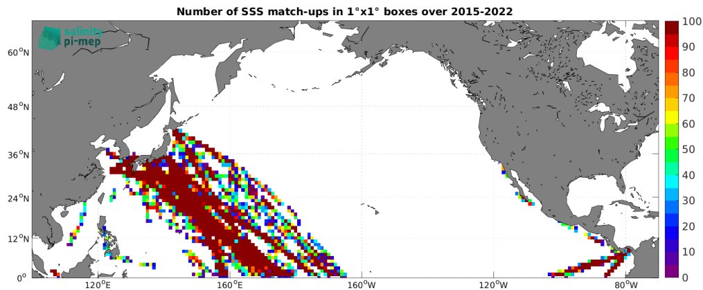
Figure 5: Number of SSS match-ups between TSG (LEGOS-DM) SSS and the SMAP SSS L2 v5.0 (JPL) SSS product for the North Pacific Ocean Pi-MEP region over 1^\circ \times 1^\circ boxes and for the full satellite product period.
