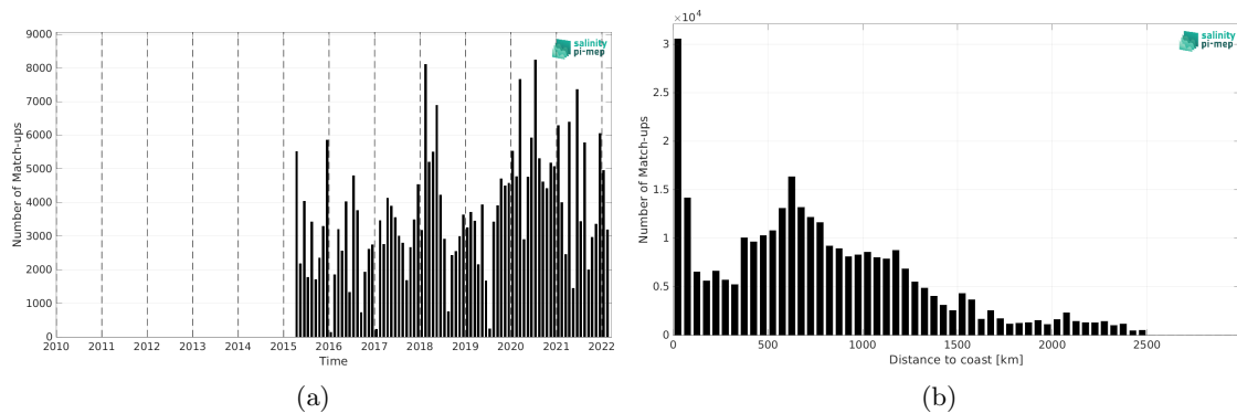
Figure 2: Number of match-ups between TSG (LEGOS-DM) and SMAP SSS L2 v5.0 (JPL) SSS as a function of time (a) and as function of the distance to coast (b) over the North Pacific Ocean Pi-MEP region and for the full satellite product period.
