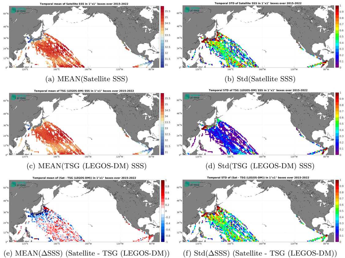
Figure 7: Temporal mean (left) and Std (right) of SSS from SMAP SSS L2 v5.0 (JPL) (top), TSG (LEGOS-DM) (middle), and of \Delta SSS (Satellite - TSG (LEGOS-DM)). Only match-up pairs are used to generate these maps.
