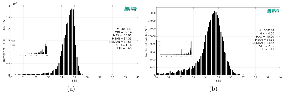
Figure 3: Histograms of SSS from TSG (LEGOS-DM) (a) and SMAP SSS L2 v5.0 (JPL) (b) considering all match-up pairs per bins of 0.1 over the North Pacific Ocean Pi-MEP region and for the full satellite product period.
