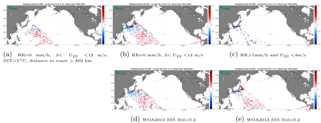
Figure 14: Temporal mean gridded over spatial boxes of size 1^\circ \times 1^\circ of \Delta\text{SSS} (SMAP SSS L2 v5.0 (JPL) - TSG (LEGOS-DM)) for 5 different subdatasets corresponding to: RR=0 mm/h, 3 < U_{10} < 12 m/s, SST > 5°C, distance to coast > 800 km (a), RR=0 mm/h, 3 < U_{10} < 12 m/s (b), RR > 1mm/h and U_{10} < 4 m/s (c), WOA2013 SSS Std < 0.2 (d), WOA2013 SSS Std > 0.2 (e).
