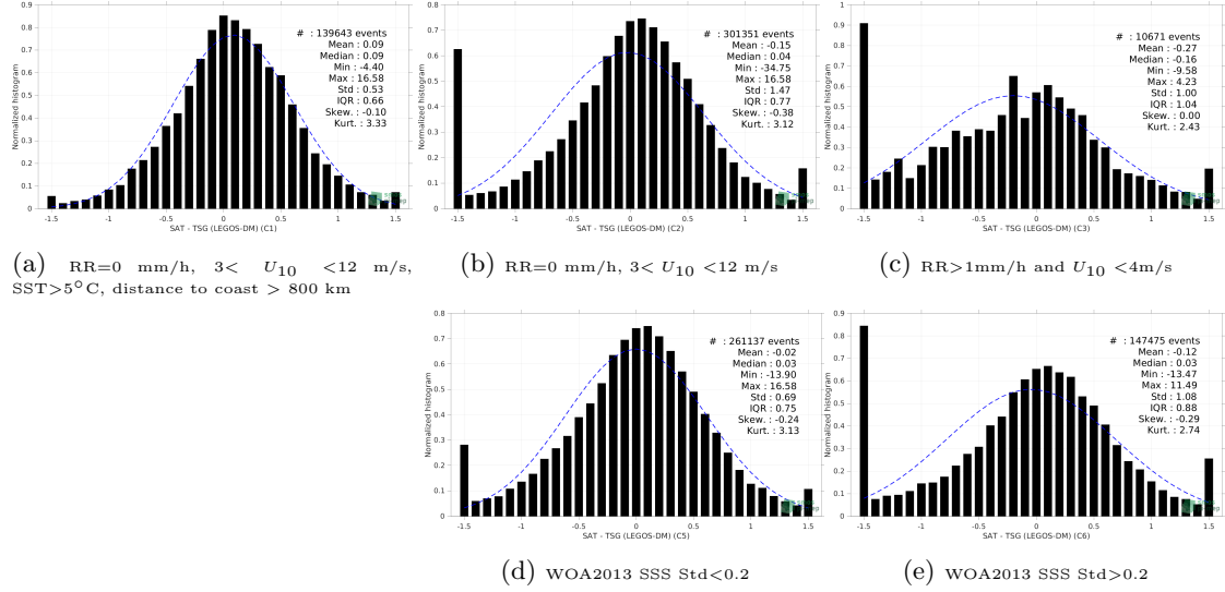
Figure 13: Normalized histogram of \Delta SSS (SMAP SSS L2 v5.0 (JPL) - TSG (LEGOS-DM)) for 5 different subdatasets corresponding to: RR=0 mm/h, 3 < U_{10} < 12 m/s, SST > 5°C, distance to coast > 800 km (a), RR=0 mm/h, 3 < U_{10} < 12 m/s (b), RR > 1mm/h and U_{10} < 4 m/s (c), WOA2013 SSS Std < 0.2 (d), WOA2013 SSS Std > 0.2 (e).
