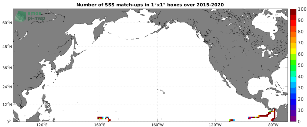
Figure 4: Number of SSS match-ups between TSG (GOSUD-Research-vessel) SSS and the SMAP SSS L2 v5.0 (JPL) SSS product for the North Pacific Ocean Pi-MEP region over 1^\circ \times 1^\circ boxes and for the full satellite product period.
