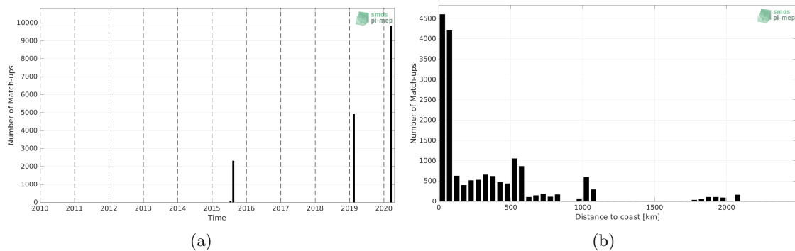
Figure 1: Number of match-ups between TSG (GOSUD-Research-vessel) and SMAP SSS L2 v5.0 (JPL) SSS as a function of time (a) and as function of the distance to coast (b) over the North Pacific Ocean Pi-MEP region and for the full satellite product period.
