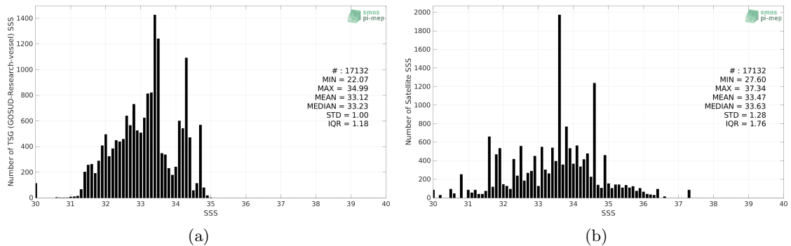
Figure 2: Histograms of SSS from TSG (GOSUD-Research-vessel) (a) and SMAP SSS L2 v5.0 (JPL) (b) considering all match-up pairs per bins of 0.1 over the North Pacific Ocean Pi-MEP region and for the full satellite product period.
