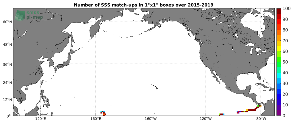
Figure 4: Number of SSS match-ups between TSG (GOSUD-Research-vessel) SSS and the SMAP SSS L2 v5.0 (JPL) SSS product for the North Pacific Ocean Pi-MEP region over 1^\circ \times 1^\circ boxes and for the full satellite product period.
