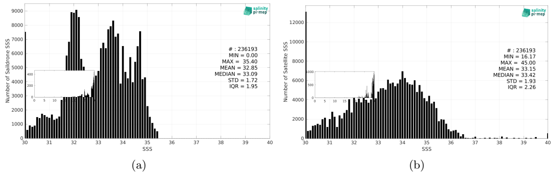
Figure 3: Histograms of SSS from Sairdrone (a) and SMAP SSS L2 v5.0 (JPL) (b) considering all match-up pairs per bins of 0.1 over the North Pacific Ocean Pi-MEP region and for the full satellite product period.
