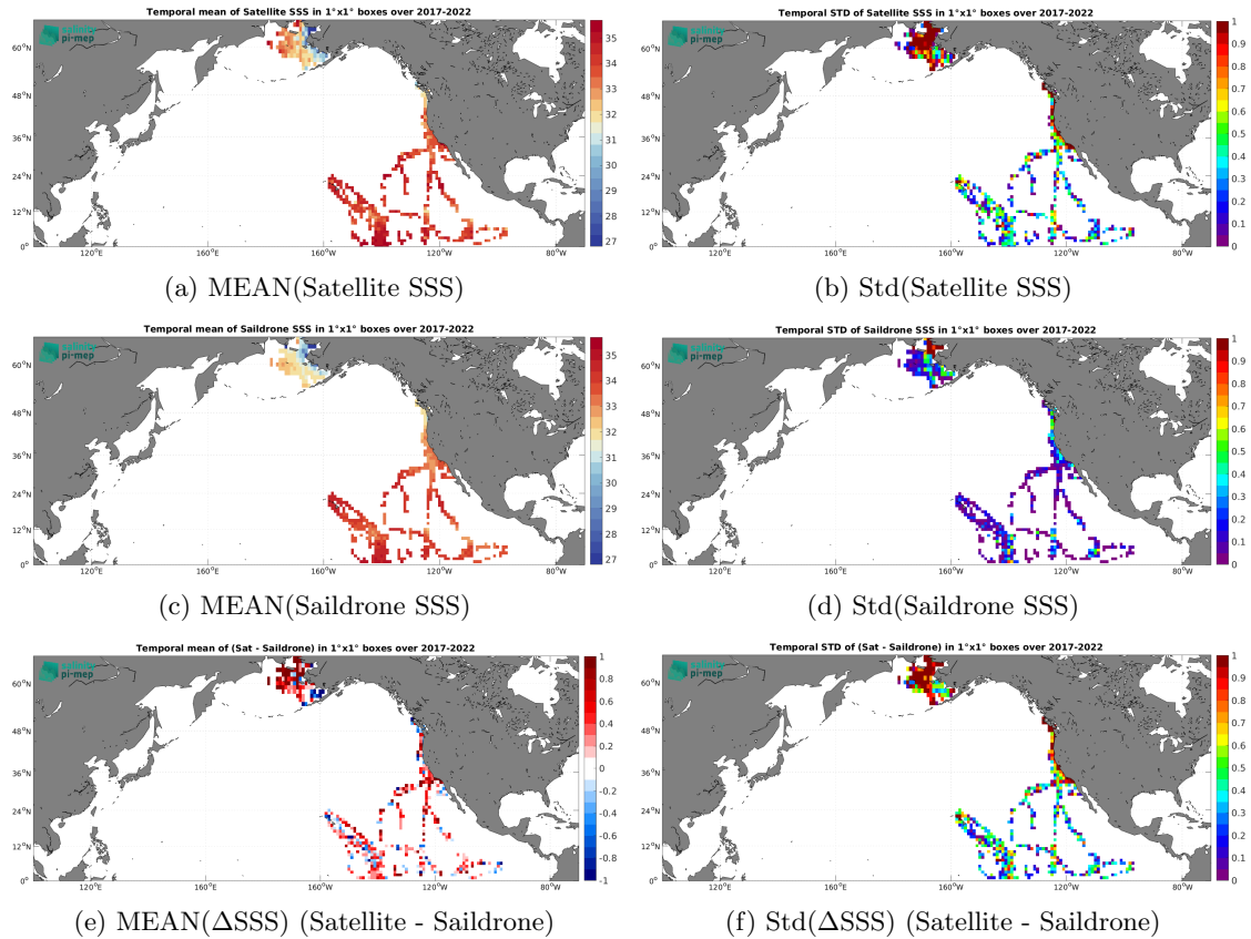
Figure 7: Temporal mean (left) and Std (right) of SSS from SMAP SSS L2 v5.0 (JPL) (top), Saildrone (middle), and of \Delta SSS (Satellite - Saildrone). Only match-up pairs are used to generate these maps.
