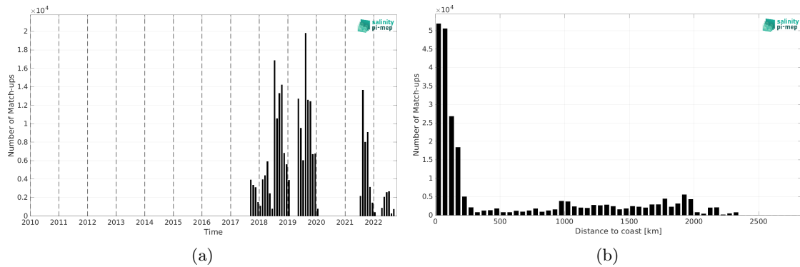
Figure 2: Number of match-ups between Sairdrone and SMAP SSS L2 v5.0 (JPL) SSS as a function of time (a) and as function of the distance to coast (b) over the North Pacific Ocean Pi-MEP region and for the full satellite product period.
