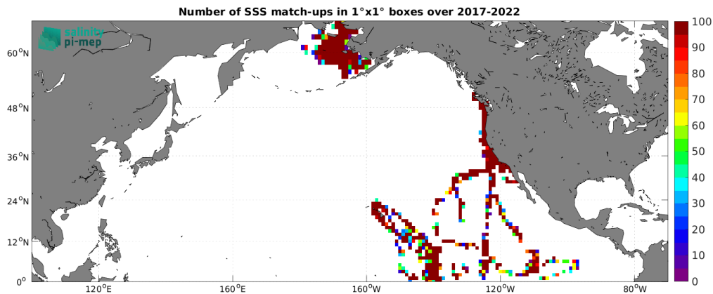
Figure 5: Number of SSS match-ups between Saildrone SSS and the SMAP SSS L2 v5.0 (JPL) SSS product for the North Pacific Ocean Pi-MEP region over 1^\circ \times 1^\circ boxes and for the full satellite product period.
