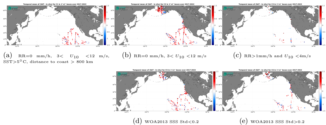
Figure 14: Temporal mean gridded over spatial boxes of size 1^\circ \times 1^\circ of \Delta SSS (SMAP SSS L2 v5.0 (JPL) - Saldrone) for 5 different subdatasets corresponding to: RR=0 mm/h, 3 < U_{10} < 12 m/s, SST > 5^\circ\text{C} , distance to coast > 800 km (a), RR=0 mm/h, 3 < U_{10} < 12 m/s (b), RR > 1 mm/h and U_{10} < 4 m/s (c), WOA2013 SSS Std < 0.2 (d), WOA2013 SSS Std > 0.2 (e).
