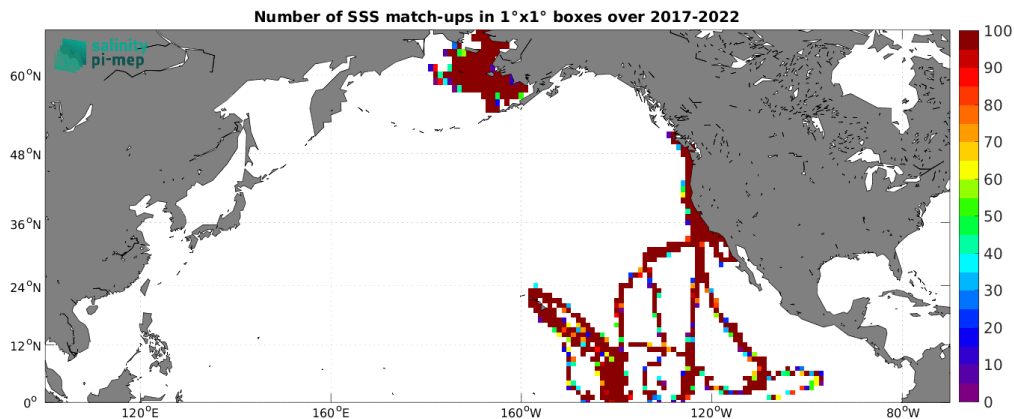
Figure 4: Number of SSS match-ups between Saildrone SSS and the SMAP SSS L2 v5.0 (JPL) SSS product for the North Pacific Ocean Pi-MEP region over 1^\circ \times 1^\circ boxes and for the full satellite product period.
