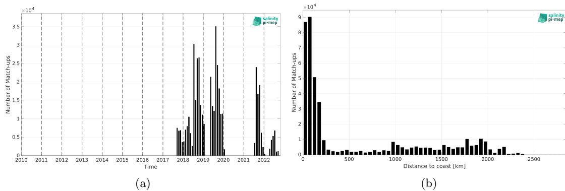
Figure 1: Number of match-ups between Sairdrone and SMAP SSS L2 v5.0 (JPL) SSS as a function of time (a) and as function of the distance to coast (b) over the North Pacific Ocean Pi-MEP region and for the full satellite product period.
