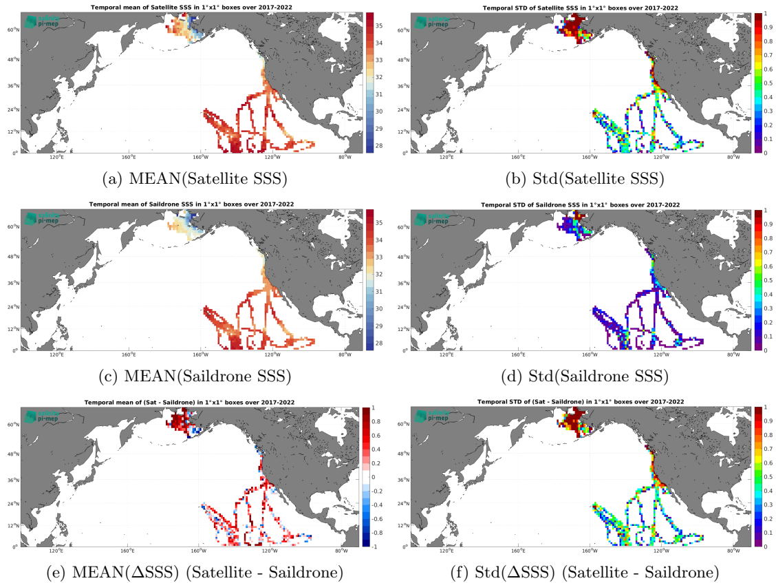
Figure 6: Temporal mean (left) and Std (right) of SSS from SMAP SSS L2 v5.0 (JPL) (top), Saildrone (middle), and of \Delta SSS (Satellite - Saildrone). Only match-up pairs are used to generate these maps.
