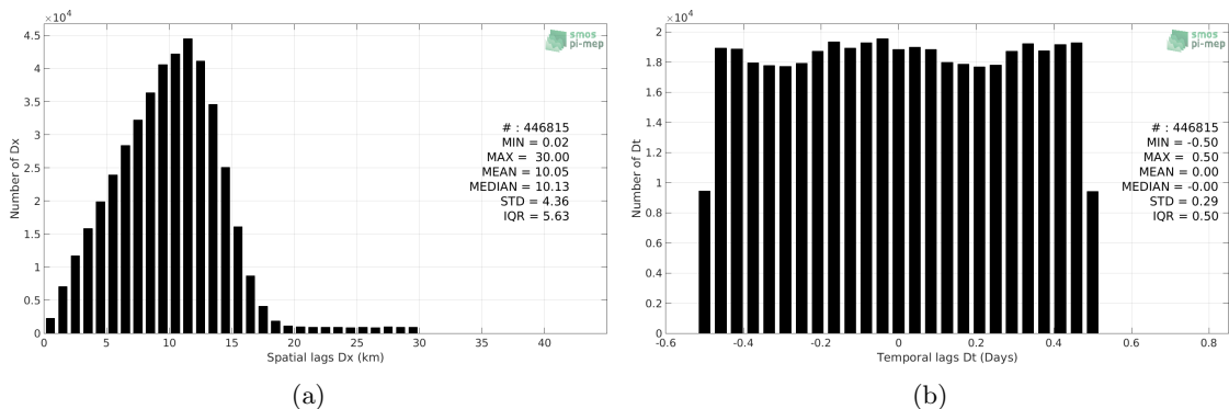
Figure 4: Histograms of the spatial (a) and temporal (b) lags between the time of the Surface drifters measurements and the date of the corresponding SMAP SSS L2 v5.0 (JPL) SSS product.
