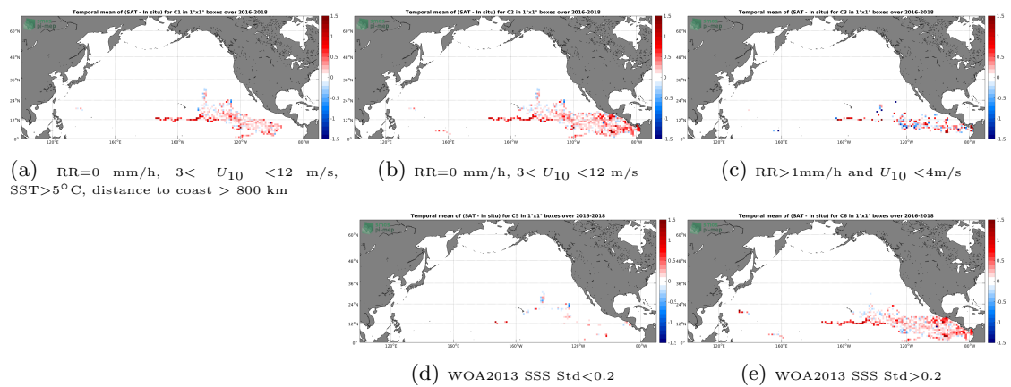
Figure 11: Temporal mean gridded over spatial boxes of size 1°x1° of \Delta SSS (SMAP SSS L2 v5.0 (JPL) - Surface drifters) for 5 different subdatasets corresponding to:RR=0 mm/h, 3 < U_{10} < 12 m/s, SST>5°C, distance to coast > 800 km (a), RR=0 mm/h, 3 < U_{10} < 12 m/s (b), RR>1mm/h and U_{10} < 4 m/s (c), WOA2013 SSS Std<0.2 (d), WOA2013 SSS Std>0.2 (e).
