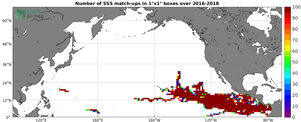
Figure 3: Number of SSS match-ups between Surface drifters SSS and the SMAP SSS L2 v5.0 (JPL) SSS product for the North Pacific Ocean Pi-MEP region over 1°x1° boxes and for the full satellite product period.
