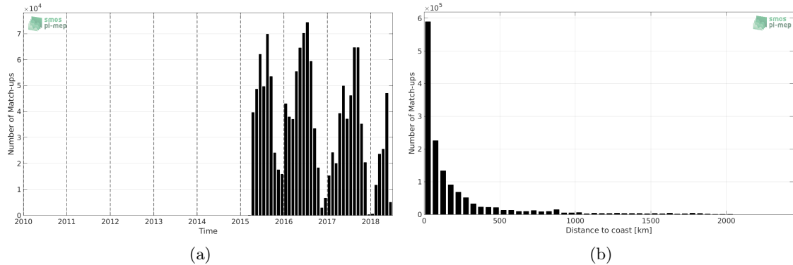
Figure 1: Number of match-ups between TSG-SAMOS and SMAP-L2-JPL-V4 SSS as a function of time (a) and as function of the distance to coast (b) over the North Pacific Ocean Pi-MEP region and for the full satellite product period.
