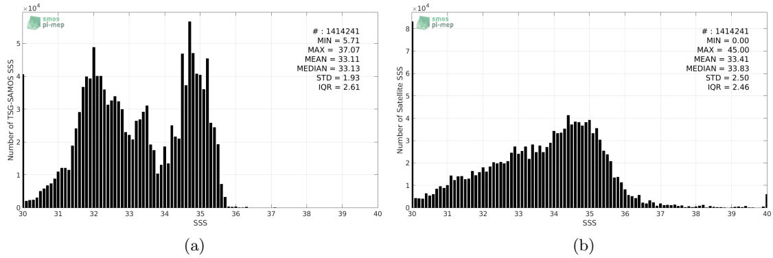
Figure 2: Histograms of SSS from TSG-SAMOS (a) and SMAP-L2-JPL-V4 (b) considering all match-up pairs per bins of 0.1 over the North Pacific Ocean Pi-MEP region and for the full satellite product period.
