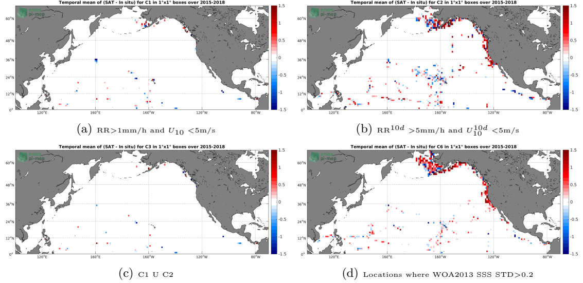
Figure 12: Temporal mean gridded over spatial boxes of size 1^\circ \times 1^\circ of \Delta SSS (SMAP-L2-JPL-V4 - TSG-SAMOS) for 4 different subdatasets corresponding to: RR > 1mm/h and U_{10} < 5\text{m/s} (a), RR^{10d} > 5\text{mm/h} and U_{10}^{10d} < 5\text{m/s} (b), C1 U C2 (c), Locations where WOA2013 SSS STD > 0.2 (d).
