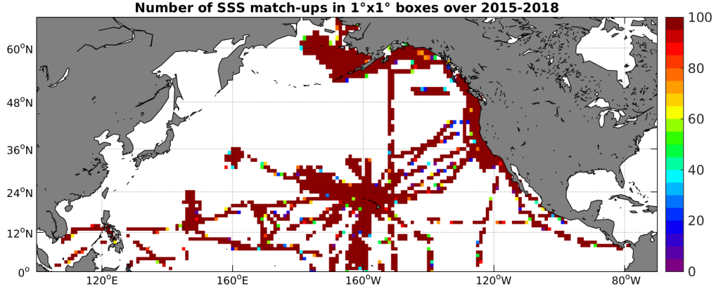
Figure 4: Number of SSS match-ups between TSG-SAMOS SSS and the SMAP-L2-JPL-V4 SSS product for the North Pacific Ocean Pi-MEP region over 1^\circ \times 1^\circ boxes and for the full satellite product period.
