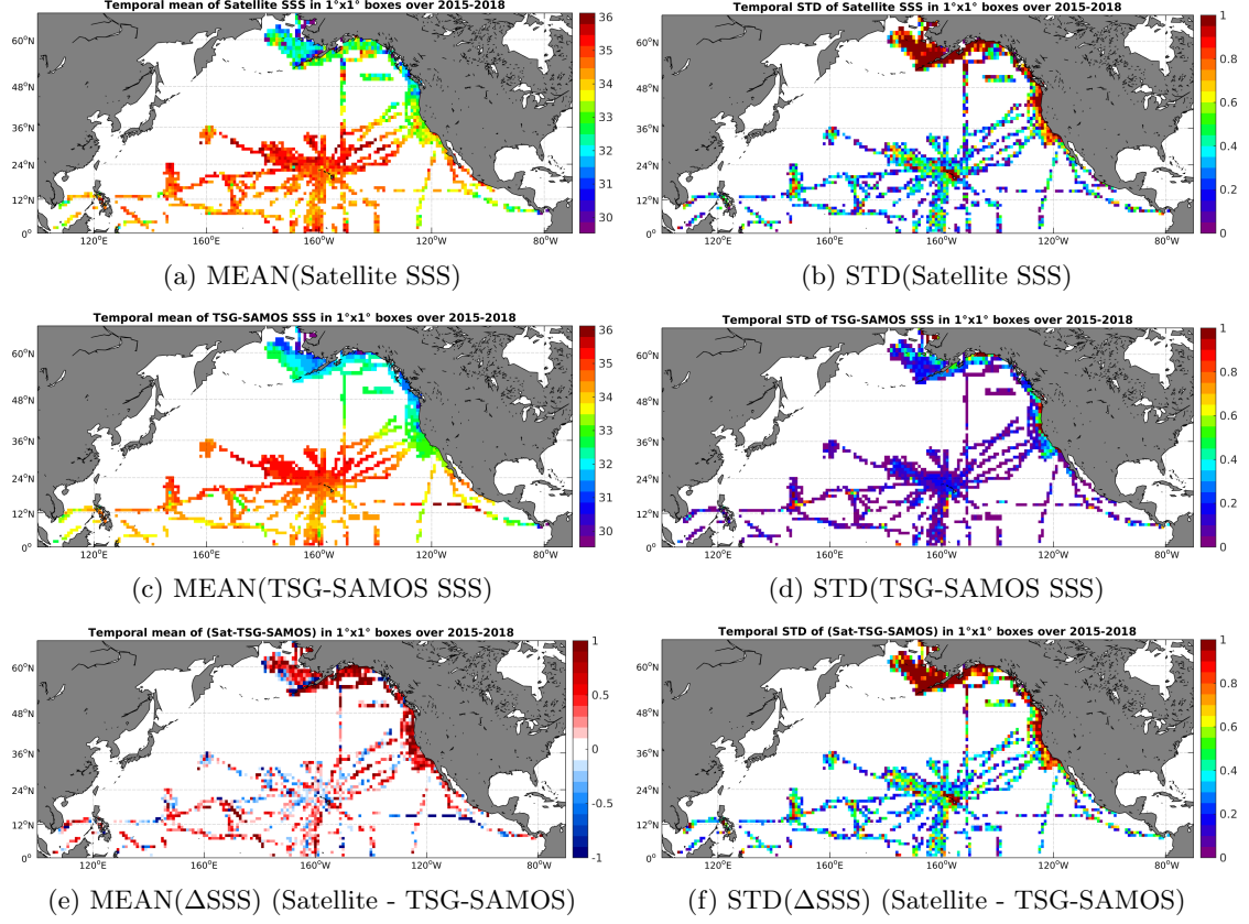
Figure 6: Temporal mean (left) and STD (right) of SSS from SMAP-L2-JPL-V4 (top), TSG-SAMOS (middle), and of \Delta SSS (Satellite - TSG-SAMOS). Only match-up pairs are used to generate these maps.
