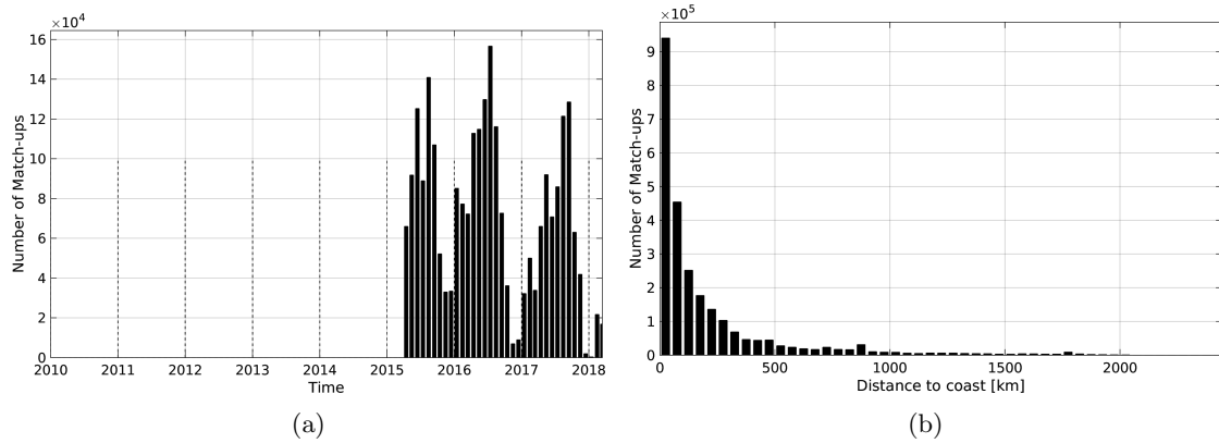
Figure 1: Number of match-ups between TSG-SAMOS and SMAP-L2-JPL-V4 SSS as a function of time (a) and as function of the distance to coast (b) over the North Pacific Ocean Pi-MEP region and for the full satellite product period.
