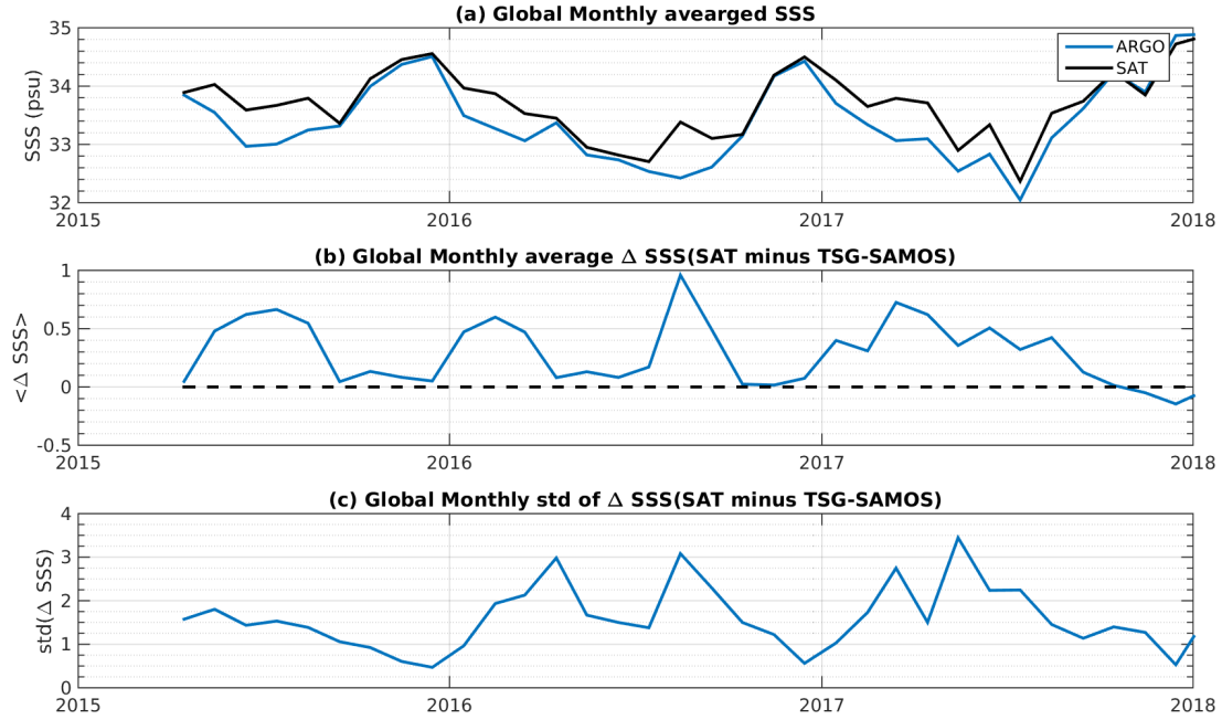
Figure 7: Time series of the monthly averaged mean SSS (top), mean \Delta SSS (Satellite - TSG-SAMOS) and STD of \Delta SSS (Satellite - TSG-SAMOS) over the North Pacific Ocean Pi-MEP region considering all match-ups collected by the Pi-MEP platform.
