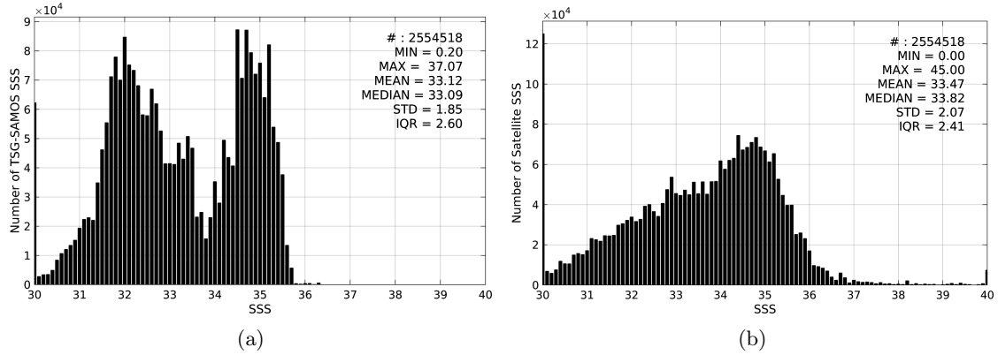
Figure 2: Histograms of SSS from TSG-SAMOS (a) and SMAP-L2-JPL-V4 (b) considering all match-up pairs per bins of 0.1 over the North Pacific Ocean Pi-MEP region and for the full satellite product period.
