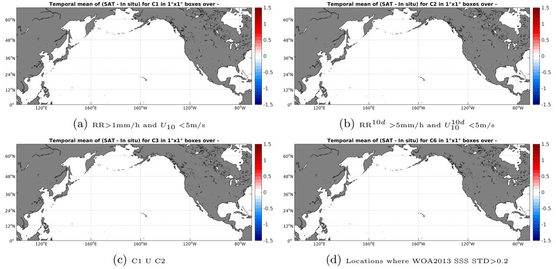
Figure 12: Temporal mean gridded over spatial boxes of size 1^\circ \times 1^\circ of \Delta SSS (SMAP-L2-JPL-V4 - TSG-GOSUD-Sailing-ship) for 4 different subdatasets corresponding to: RR > 1mm/h and U_{10} < 5 m/s (a), RR^{10d} > 5 mm/h and U_{10}^{10d} < 5 m/s (b), C1 U C2 (c), Locations where WOA2013 SSS STD > 0.2 (d).
