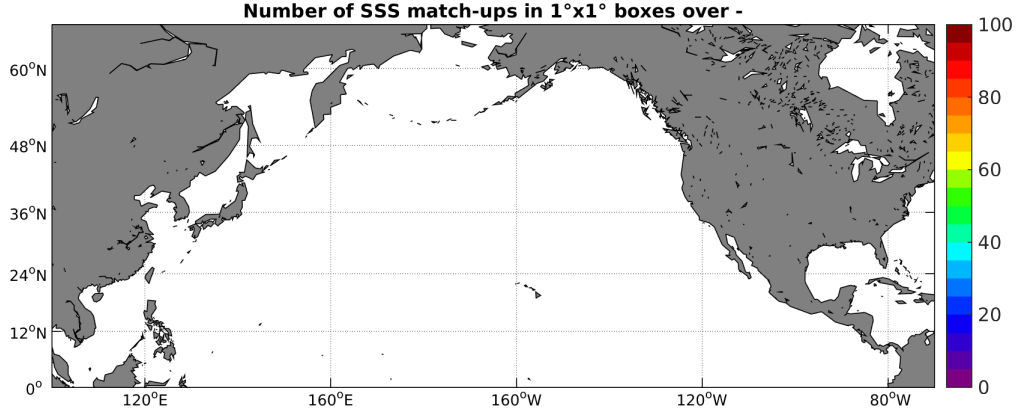
Figure 4: Number of SSS match-ups between TSG-GOSUD-Sailing-ship SSS and the SMAP-L2-JPL-V4 SSS product for the North Pacific Ocean Pi-MEP region over 1^\circ \times 1^\circ boxes and for the full satellite product period.
