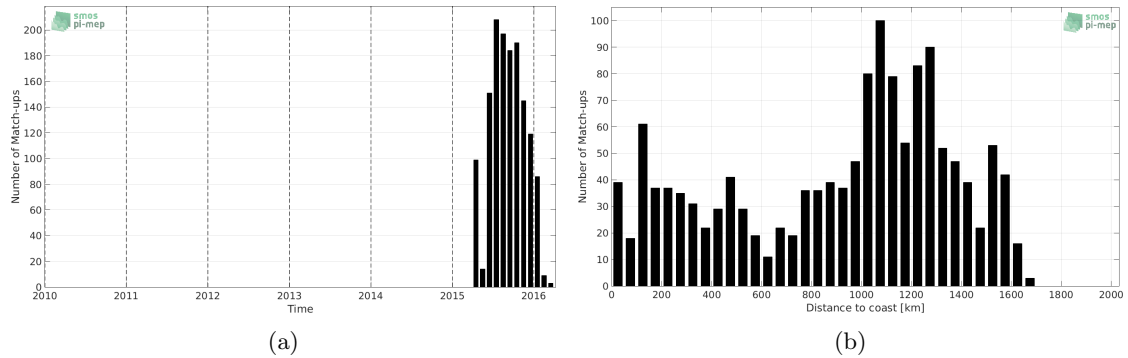
Figure 1: Number of match-ups between Sea mammals and SMAP-L2-JPL-V4 SSS as a function of time (a) and as function of the distance to coast (b) over the North Pacific Ocean Pi-MEP region and for the full satellite product period.
