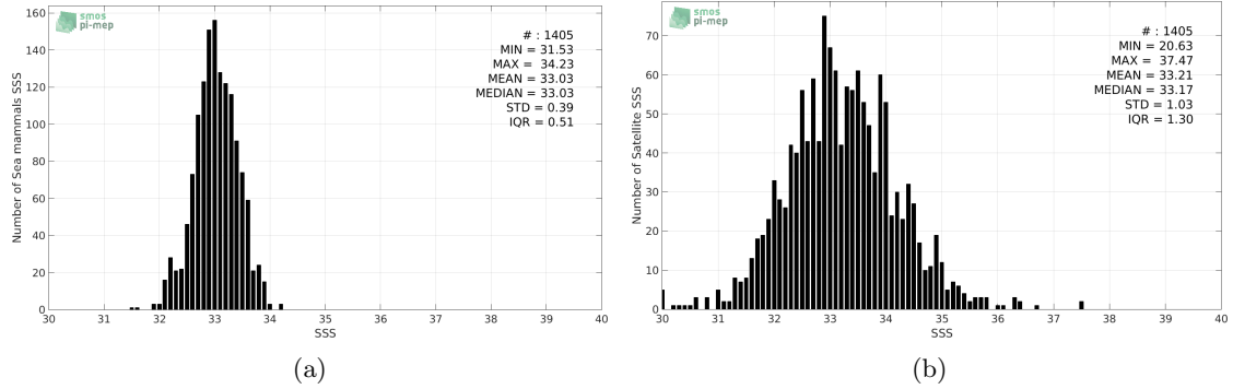
Figure 2: Histograms of SSS from Sea mammals (a) and SMAP-L2-JPL-V4 (b) considering all match-up pairs per bins of 0.1 over the North Pacific Ocean Pi-MEP region and for the full satellite product period.
