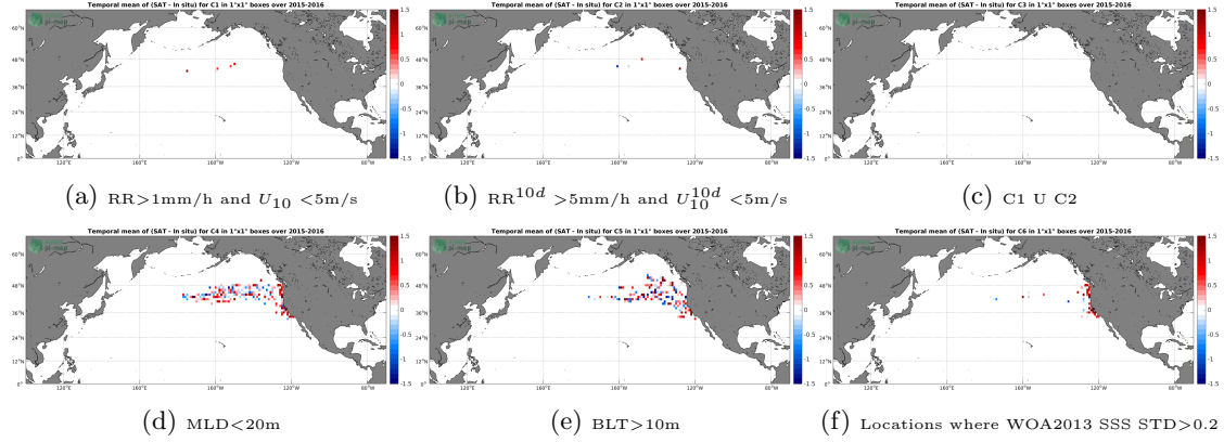
Figure 12: Temporal mean gridded over spatial boxes of size 1^\circ \times 1^\circ of \Delta\text{SSS} (SMAP-L2-JPL-V4 - Sea mammals) for 6 different subdatasets corresponding to: RR > 1\text{mm/h} and U_{10} < 5\text{m/s} (a), RR^{10d} > 5\text{mm/h} and U_{10}^{10d} < 5\text{m/s} (b), C1 U C2 (c), MLD < 20\text{m} (d), BLT > 10\text{m} (e), Locations where WOA2013 SSS STD > 0.2 (f).
