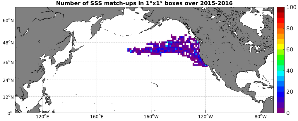
Figure 4: Number of SSS match-ups between Sea mammals SSS and the SMAP-L2-JPL-V4 SSS product for the North Pacific Ocean Pi-MEP region over 1^\circ \times 1^\circ boxes and for the full satellite product period.
