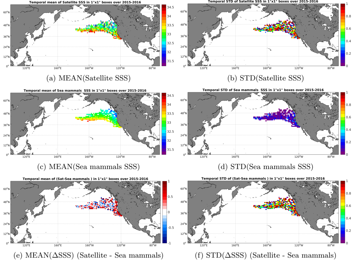
Figure 6: Temporal mean (left) and STD (right) of SSS from SMAP-L2-JPL-V4 (top), Sea mammals (middle), and of \Delta SSS (Satellite - Sea mammals). Only match-up pairs are used to generate these maps.
