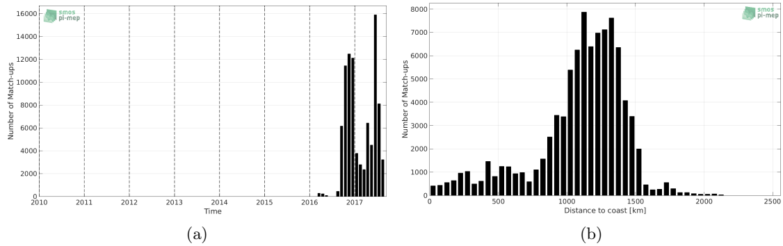
Figure 1: Number of match-ups between Surface drifters and SMAP-L2-JPL-V4 SSS as a function of time (a) and as function of the distance to coast (b) over the North Pacific Ocean Pi-MEP region and for the full satellite product period.
