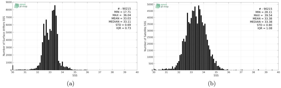
Figure 2: Histograms of SSS from Surface drifters (a) and SMAP-L2-JPL-V4 (b) considering all match-up pairs per bins of 0.1 over the North Pacific Ocean Pi-MEP region and for the full satellite product period.
