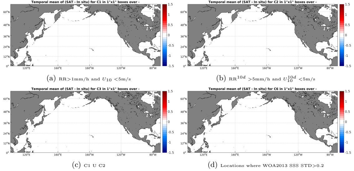
Figure 11: Temporal mean gridded over spatial boxes of size 1^\circ \times 1^\circ of \Delta SSS (SMAP-L2-JPL-V4 - Surface drifters) for 4 different subdatasets corresponding to: RR > 1mm/h and U_{10} < 5 m/s (a), RR^{10d} > 5 mm/h and U_{10}^{10d} < 5 m/s (b), C1 U C2 (c), Locations where WOA2013 SSS STD > 0.2 (d).
