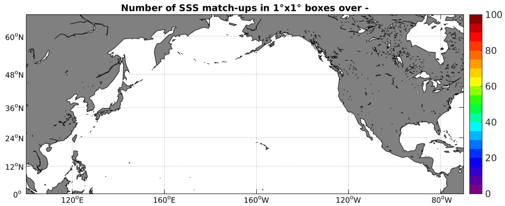
Figure 3: Number of SSS match-ups between Surface drifters SSS and the SMAP-L2-JPL-V4 SSS product for the North Pacific Ocean Pi-MEP region over 1^\circ \times 1^\circ boxes and for the full satellite product period.
