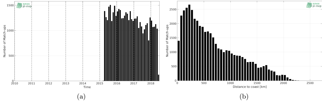
Figure 1: Number of match-ups between Argo and SMAP-L2-JPL-V4 SSS as a function of time (a) and as function of the distance to coast (b) over the North Pacific Ocean Pi-MEP region and for the full satellite product period.
