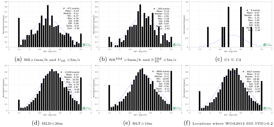
Figure 13: Normalized histogram of \Delta SSS (SMAP-L2-JPL-V4 - Argo) for 6 different subdatasets corresponding to: RR>1\text{mm/h} and U_{10}<5\text{m/s} (a), RR^{10d}>5\text{mm/h} and U_{10}^{10d}<5\text{m/s} (b), C1 U C2 (c), MLD<20\text{m} (d), BLT>10\text{m} (e), Locations where WOA2013 SSS STD>0.2 (f).
