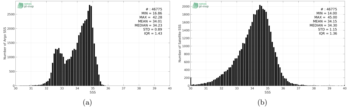
Figure 2: Histograms of SSS from Argo (a) and SMAP-L2-JPL-V4 (b) considering all match-up pairs per bins of 0.1 over the North Pacific Ocean Pi-MEP region and for the full satellite product period.
