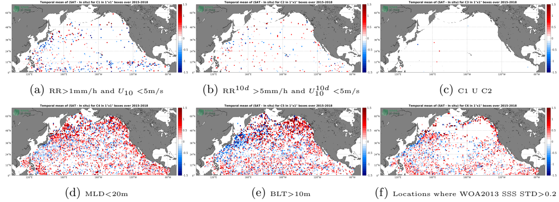
Figure 12: Temporal mean gridded over spatial boxes of size 1^\circ \times 1^\circ of \Delta SSS (SMAP-L2-JPL-V4 - Argo) for 6 different subdatasets corresponding to: RR>1\text{mm/h} and U_{10}<5\text{m/s} (a), RR^{10d}>5\text{mm/h} and U_{10}^{10d}<5\text{m/s} (b), C1 U C2 (c), MLD<20\text{m} (d), BLT>10\text{m} (e), Locations where WOA2013 SSS STD>0.2 (f).
