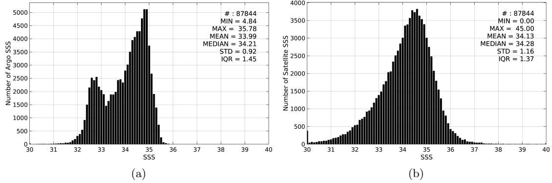
Figure 2: Histograms of SSS from Argo (a) and SMAP-L2-JPL-V4 (b) considering all match-up pairs per bins of 0.1 over the North Pacific Ocean Pi-MEP region and for the full satellite product period.
