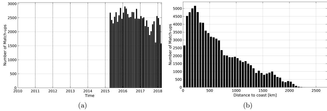
Figure 1: Number of match-ups between Argo and SMAP-L2-JPL-V4 SSS as a function of time (a) and as function of the distance to coast (b) over the North Pacific Ocean Pi-MEP region and for the full satellite product period.
