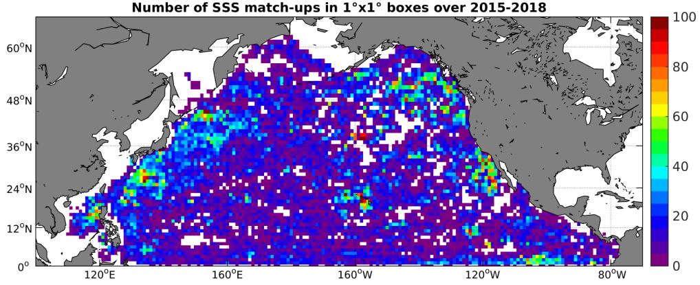
Figure 4: Number of SSS match-ups between Argo SSS and the SMAP-L2-JPL-V4 SSS product for the North Pacific Ocean Pi-MEP region over 1^\circ \times 1^\circ boxes and for the full satellite product period.
