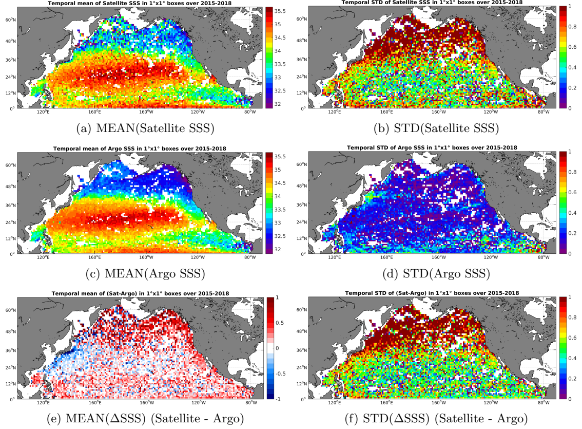
Figure 6: Temporal mean (left) and STD (right) of SSS from SMAP-L2-JPL-V4 (top), Argo (middle), and of \Delta SSS (Satellite - Argo). Only match-up pairs are used to generate these maps.
