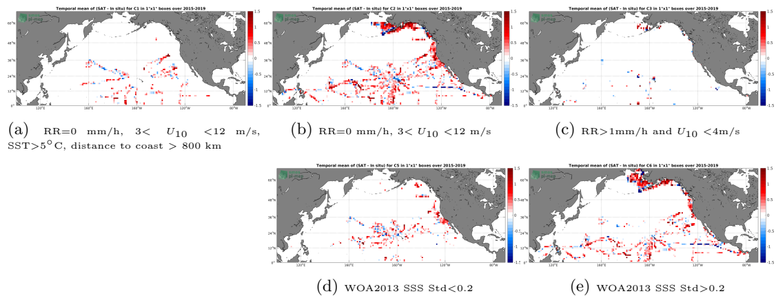
Figure 12: Temporal mean gridded over spatial boxes of size 1^\circ \times 1^\circ of \Delta SSS (SMAP-L2-JPL-V4.2 - TSG-SAMOS) for 5 different subdatasets corresponding to:RR=0 mm/h, 3 < U_{10} < 12 m/s, SST > 5^\circ\text{C} , distance to coast > 800 km (a), RR=0 mm/h, 3 < U_{10} < 12 m/s (b), RR > 1 mm/h and U_{10} < 4 m/s (c), WOA2013 SSS Std < 0.2 (d), WOA2013 SSS Std > 0.2 (e).
