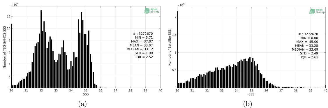
Figure 2: Histograms of SSS from TSG-SAMOS (a) and SMAP-L2-JPL-V4.2 (b) considering all match-up pairs per bins of 0.1 over the North Pacific Ocean Pi-MEP region and for the full satellite product period.
