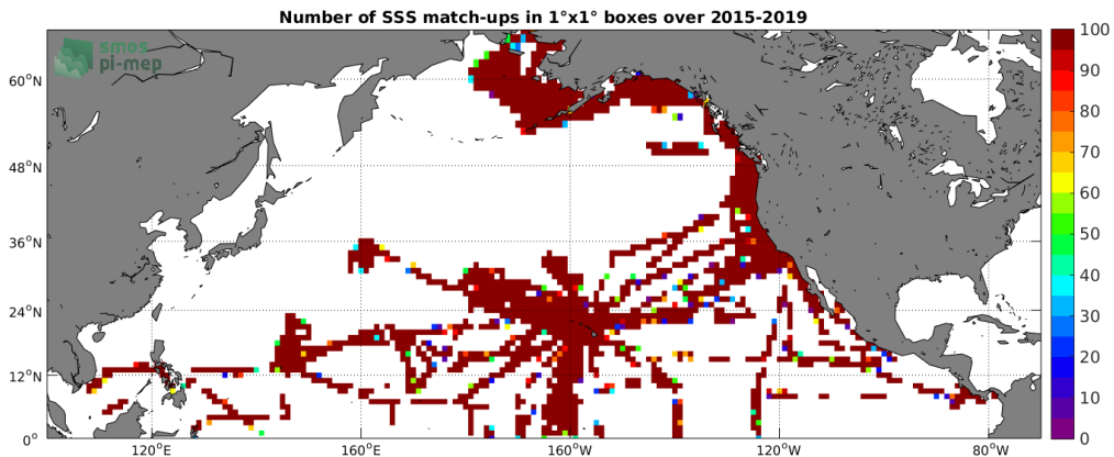
Figure 4: Number of SSS match-ups between TSG-SAMOS SSS and the SMAP-L2-JPL-V4.2 SSS product for the North Pacific Ocean Pi-MEP region over 1^\circ \times 1^\circ boxes and for the full satellite product period.
