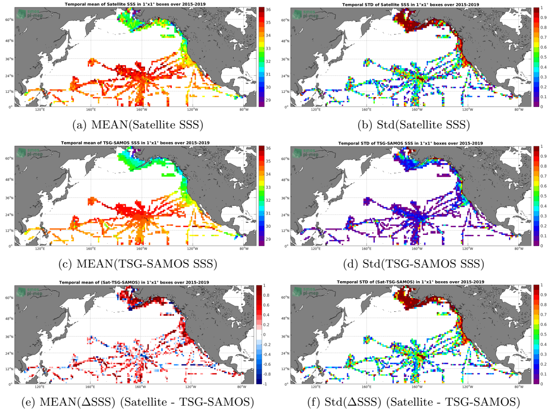
Figure 6: Temporal mean (left) and Std (right) of SSS from SMAP-L2-JPL-V4.2 (top), TSG-SAMOS (middle), and of \Delta SSS (Satellite - TSG-SAMOS). Only match-up pairs are used to generate these maps.
