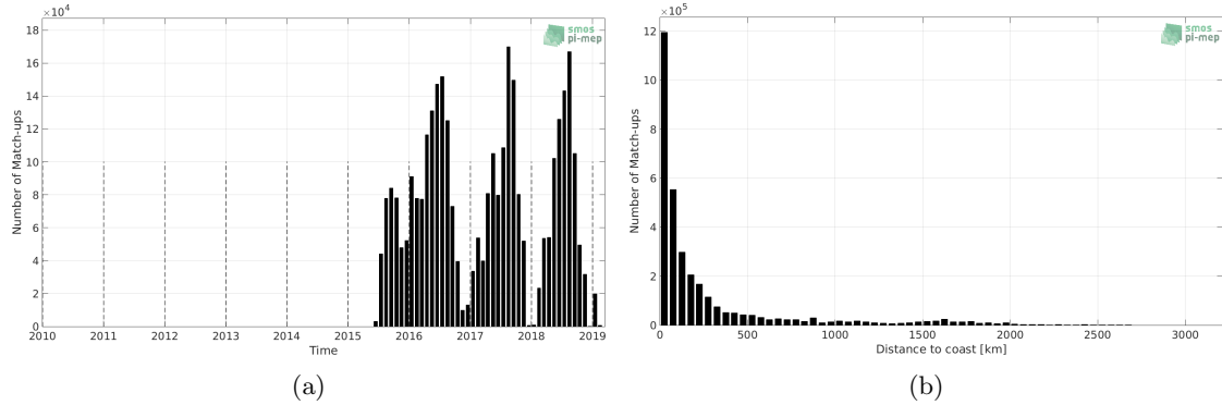
Figure 1: Number of match-ups between TSG-SAMOS and SMAP-L2-JPL-V4.2 SSS as a function of time (a) and as function of the distance to coast (b) over the North Pacific Ocean Pi-MEP region and for the full satellite product period.
