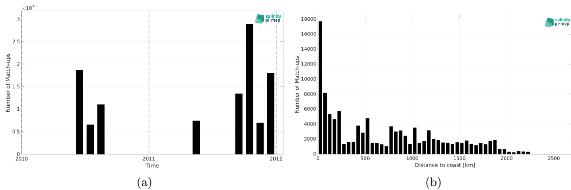
Figure 2: Number of match-ups between TSG (GOSUD-Sailing-ship) and ISAS v7 - Monthly (Ifremer-LOPS-CMEMS) SSS as a function of time (a) and as function of the distance to coast (b) over the North Pacific Ocean Pi-MEP region and for the full satellite product period.
