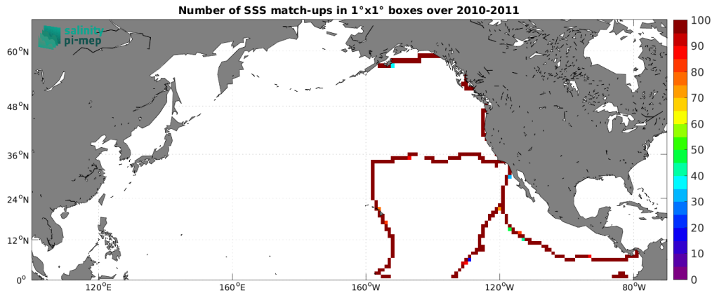
Figure 5: Number of SSS match-ups between TSG (GOSUD-Sailing-ship) SSS and the ISAS v7 - Monthly (Ifremer-LOPS-CMEMS) SSS product for the North Pacific Ocean Pi-MEP region over 1^\circ \times 1^\circ boxes and for the full satellite product period.
