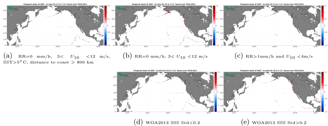
Figure 14: Temporal mean gridded over spatial boxes of size 1^\circ \times 1^\circ of \Delta SSS (ISAS - TSG (GOSUD-Sailing-ship)) for 5 different subdatasets corresponding to:RR=0 mm/h, 3 < U_{10} < 12 m/s, SST>5°C, distance to coast > 800 km (a), RR=0 mm/h, 3 < U_{10} < 12 m/s (b), RR>1mm/h and U_{10} < 4 m/s (c), WOA2013 SSS Std<0.2 (d), WOA2013 SSS Std>0.2 (e).
