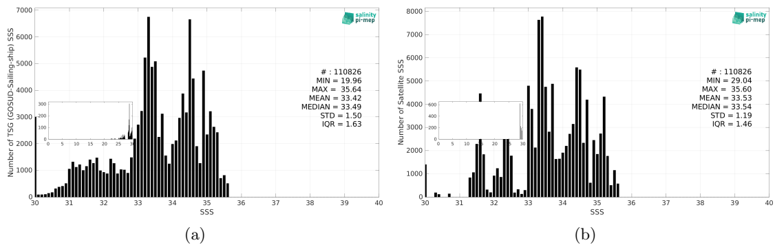
Figure 3: Histograms of SSS from TSG (GOSUD-Sailing-ship) (a) and ISAS (b) considering all match-up pairs per bins of 0.1 over the North Pacific Ocean Pi-MEP region and for the full satellite product period.
