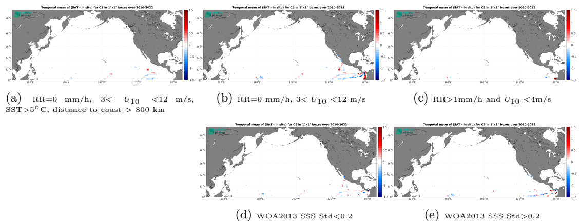
Figure 14: Temporal mean gridded over spatial boxes of size 1^\circ \times 1^\circ of \Delta SSS (ISAS v7 - Monthly (Ifremer-LOPS-CMEMS) - TSG (GOSUD-Research-vessel)) for 5 different subdatasets corresponding to:RR=0 mm/h, 3 < U_{10} < 12 m/s, SST >5^\circ\text{C} , distance to coast > 800 km (a), RR=0 mm/h, 3 < U_{10} < 12 m/s (b), RR >1 mm/h and U_{10} < 4 m/s (c), WOA2013 SSS Std <0.2 (d), WOA2013 SSS Std >0.2 (e).
