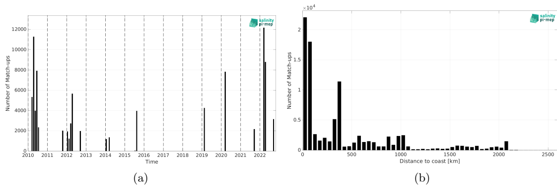
Figure 2: Number of match-ups between TSG (GOSUD-Research-vessel) and ISAS v7 - Monthly (Ifremer-LOPS-CMEMS) SSS as a function of time (a) and as function of the distance to coast (b) over the North Pacific Ocean Pi-MEP region and for the full satellite product period.
