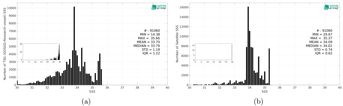
Figure 3: Histograms of SSS from TSG (GOSUD-Research-vessel) (a) and ISAS v7 - Monthly (Ifremer-LOPS-CMEMS) (b) considering all match-up pairs per bins of 0.1 over the North Pacific Ocean Pi-MEP region and for the full satellite product period.
