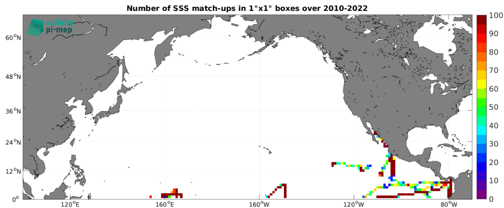
Figure 5: Number of SSS match-ups between TSG (GOSUD-Research-vessel) SSS and the ISAS v7 - Monthly (Ifremer-LOPS-CMEMS) SSS product for the North Pacific Ocean Pi-MEP region over 1^\circ \times 1^\circ boxes and for the full satellite product period.
