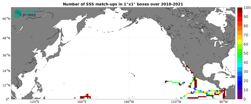
Figure 5: Number of SSS match-ups between TSG (GOSUD-Research-vessel) SSS and the ISAS SSS product for the North Pacific Ocean Pi-MEP region over 1^\circ \times 1^\circ boxes and for the full satellite product period.
