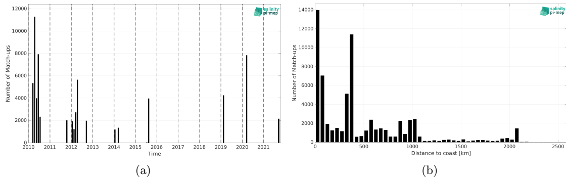
Figure 2: Number of match-ups between TSG (GOSUD-Research-vessel) and ISAS SSS as a function of time (a) and as function of the distance to coast (b) over the North Pacific Ocean Pi-MEP region and for the full satellite product period.
