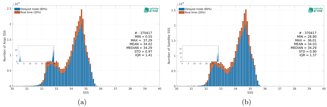
Figure 3: Histograms of SSS from Argo (a) and ISAS v7 - Monthly (Ifremer-LOPS-CMEMS) (b) considering all match-up pairs per bins of 0.1 over the North Pacific Ocean Pi-MEP region and for the full satellite product period.
