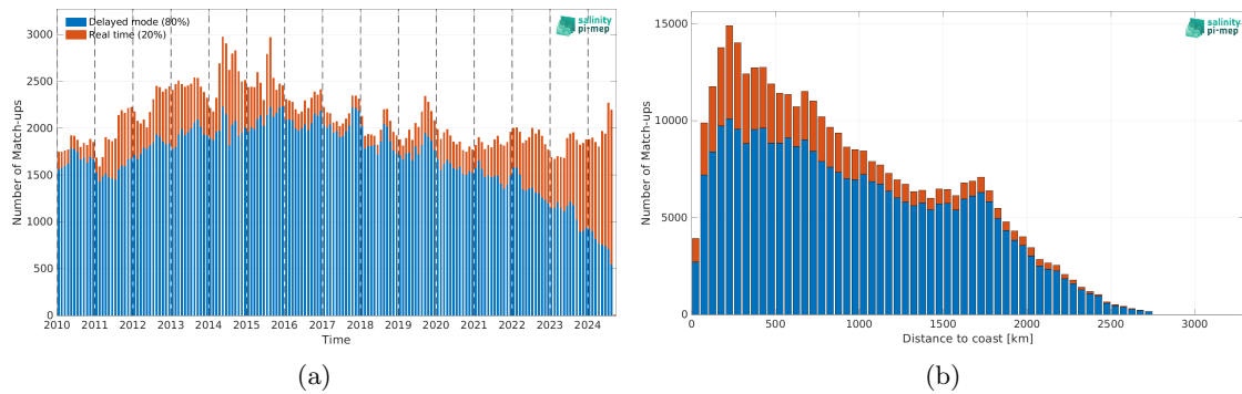
Figure 2: Number of match-ups between Argo and ISAS v7 - Monthly (Ifremer-LOPS-CMEMS) SSS as a function of time (a) and as function of the distance to coast (b) over the North Pacific Ocean Pi-MEP region and for the full satellite product period.
