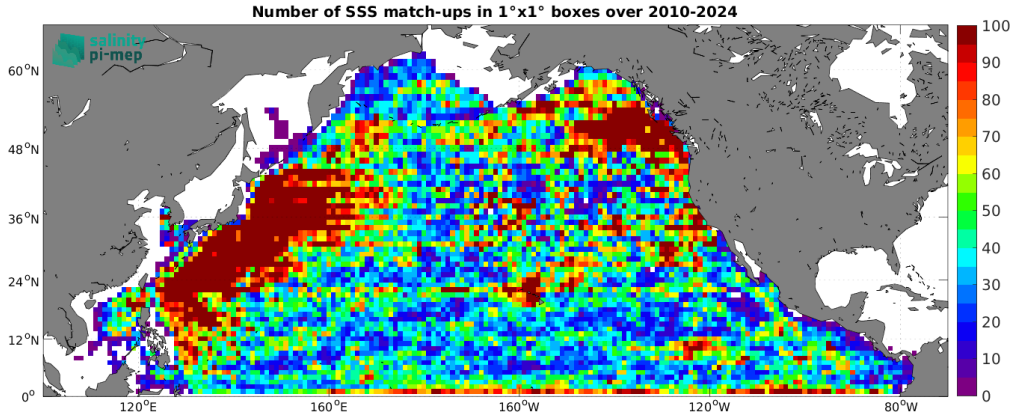
Figure 5: Number of SSS match-ups between Argo SSS and the ISAS v7 - Monthly (Ifremer-LOPS-CMEMS) SSS product for the North Pacific Ocean Pi-MEP region over 1^\circ \times 1^\circ boxes and for the full satellite product period.
