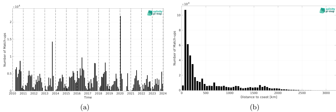
Figure 2: Number of match-ups between TSG (SAMOS) and CCI SSS L4 Merged-OI v5.5 - 7-day running (ESA) SSS as a function of time (a) and as function of the distance to coast (b) over the North Pacific Ocean Pi-MEP region and for the full satellite product period.
