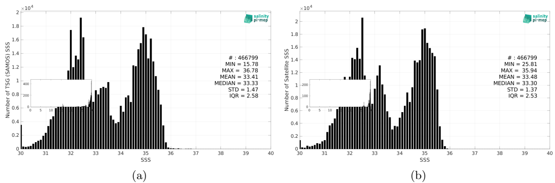
Figure 3: Histograms of SSS from TSG (SAMOS) (a) and CCI SSS L4 Merged-OI v5.5 - 7-day running (ESA) (b) considering all match-up pairs per bins of 0.1 over the North Pacific Ocean Pi-MEP region and for the full satellite product period.
