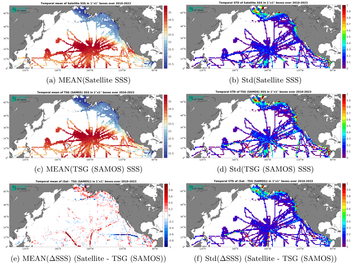
Figure 7: Temporal mean (left) and Std (right) of SSS from CCI SSS L4 Merged-OI v5.5 - 7-day running (ESA) (top), TSG (SAMOS) (middle), and of \Delta SSS (Satellite - TSG (SAMOS)). Only match-up pairs are used to generate these maps.
