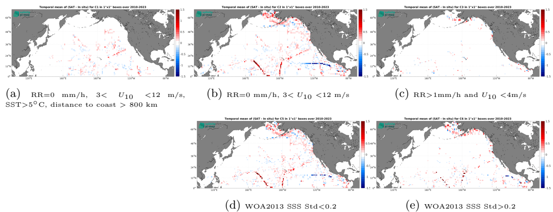
Figure 14: Temporal mean gridded over spatial boxes of size 1^\circ \times 1^\circ of \Delta\text{SSS} (CCI SSS L4 Merged-OI v5.5 - 7-day running (ESA) - TSG (SAMOS)) for 5 different subdatasets corresponding to:RR=0 mm/h, 3 < U_{10} < 12 m/s, SST>5°C, distance to coast > 800 km (a), RR=0 mm/h, 3 < U_{10} < 12 m/s (b), RR>1mm/h and U_{10} < 4 m/s (c), WOA2013 SSS Std<0.2 (d), WOA2013 SSS Std>0.2 (e).
