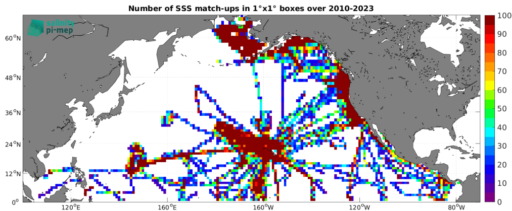
Figure 5: Number of SSS match-ups between TSG (SAMOS) SSS and the CCI SSS L4 Merged-OI v5.5 - 7-day running (ESA) SSS product for the North Pacific Ocean Pi-MEP region over 1^\circ \times 1^\circ boxes and for the full satellite product period.
