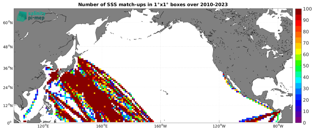
Figure 5: Number of SSS match-ups between TSG (LEGOS-DM) SSS and the CCI SSS L4 Merged-OI v5.5 - 7-day running (ESA) SSS product for the North Pacific Ocean Pi-MEP region over 1^\circ \times 1^\circ boxes and for the full satellite product period.
