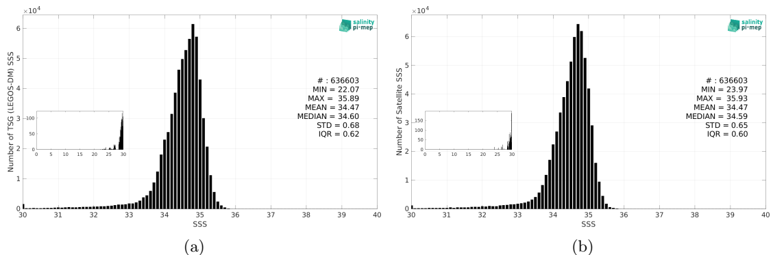
Figure 3: Histograms of SSS from TSG (LEGOS-DM) (a) and CCI SSS L4 Merged-OI v5.5 - 7-day running (ESA) (b) considering all match-up pairs per bins of 0.1 over the North Pacific Ocean Pi-MEP region and for the full satellite product period.
