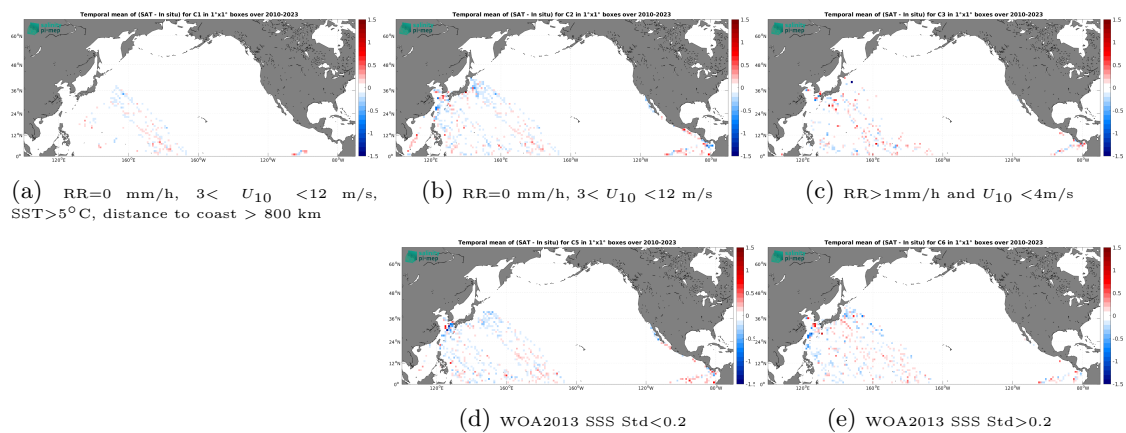
Figure 14: Temporal mean gridded over spatial boxes of size 1^\circ \times 1^\circ of \Delta\text{SSS} (CCI SSS L4 Merged-OI v5.5 - 7-day running (ESA) - TSG (LEGOS-DM)) for 5 different subdatasets corresponding to:RR=0 mm/h, 3 < U_{10} < 12 m/s, SST>5°C, distance to coast > 800 km (a), RR=0 mm/h, 3 < U_{10} < 12 m/s (b), RR>1mm/h and U_{10} < 4 m/s (c), WOA2013 SSS Std<0.2 (d), WOA2013 SSS Std>0.2 (e).
