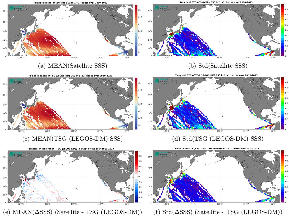
Figure 7: Temporal mean (left) and Std (right) of SSS from CCI SSS L4 Merged-OI v5.5 - 7-day running (ESA) (top), TSG (LEGOS-DM) (middle), and of \Delta SSS (Satellite - TSG (LEGOS-DM)). Only match-up pairs are used to generate these maps.
