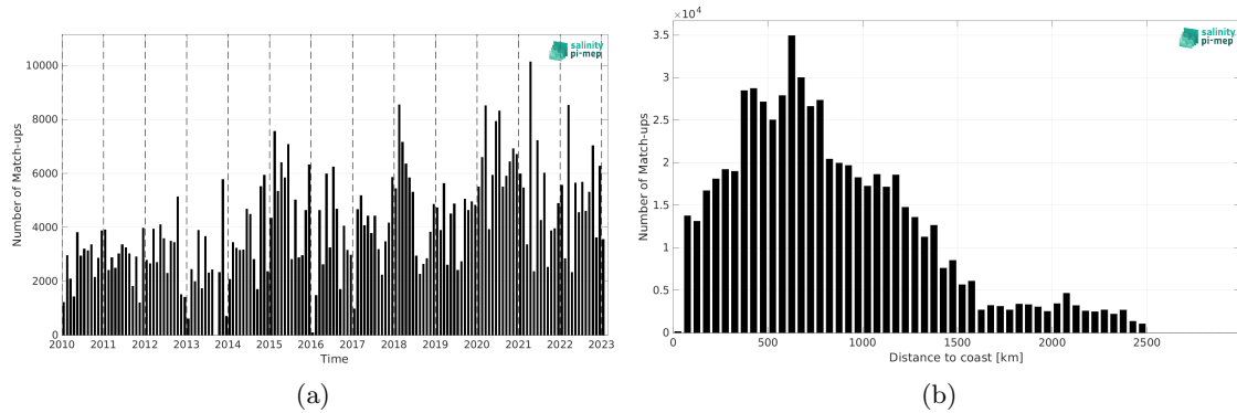
Figure 2: Number of match-ups between TSG (LEGOS-DM) and CCI SSS L4 Merged-OI v5.5 - 7-day running (ESA) SSS as a function of time (a) and as function of the distance to coast (b) over the North Pacific Ocean Pi-MEP region and for the full satellite product period.
