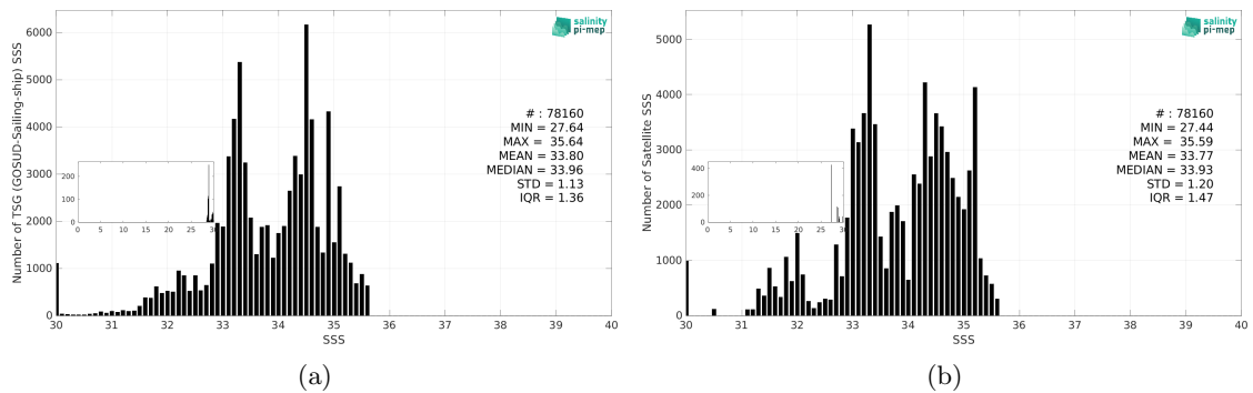
Figure 3: Histograms of SSS from TSG (GOSUD-Sailing-ship) (a) and CCI SSS L4 Merged-OI v5.5 - 7-day running (ESA) (b) considering all match-up pairs per bins of 0.1 over the North Pacific Ocean Pi-MEP region and for the full satellite product period.
