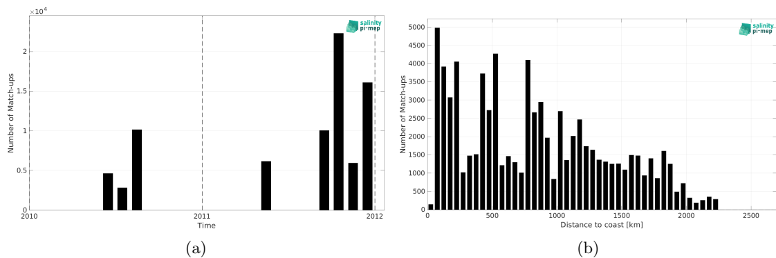
Figure 2: Number of match-ups between TSG (GOSUD-Sailing-ship) and CCI SSS L4 Merged-OI v5.5 - 7-day running (ESA) SSS as a function of time (a) and as function of the distance to coast (b) over the North Pacific Ocean Pi-MEP region and for the full satellite product period.
