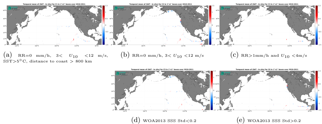
Figure 14: Temporal mean gridded over spatial boxes of size 1^\circ \times 1^\circ of \Delta\text{SSS} (CCI SSS L4 Merged-OI v5.5 - 7-day running (ESA) - TSG (GOSUD-Sailing-ship)) for 5 different subdatasets corresponding to:RR=0 mm/h, 3 < U_{10} < 12 m/s, SST >5^\circ\text{C} , distance to coast > 800 km (a), RR=0 mm/h, 3 < U_{10} < 12 m/s (b), RR >1 mm/h and U_{10} < 4 m/s (c), WOA2013 SSS Std <0.2 (d), WOA2013 SSS Std >0.2 (e).
