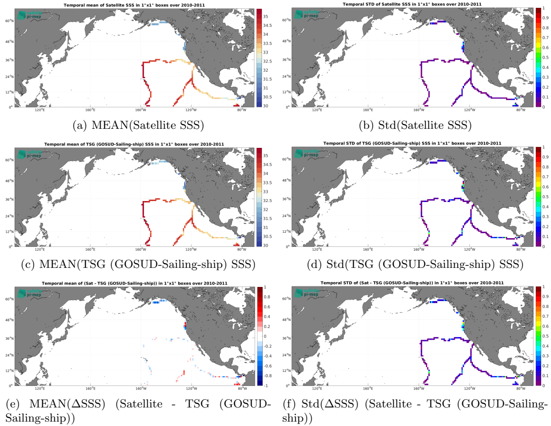
Figure 7: Temporal mean (left) and Std (right) of SSS from CCI SSS L4 Merged-OI v5.5 - 7-day running (ESA) (top), TSG (GOSUD-Sailing-ship) (middle), and of \Delta SSS (Satellite - TSG (GOSUD-Sailing-ship)). Only match-up pairs are used to generate these maps.
