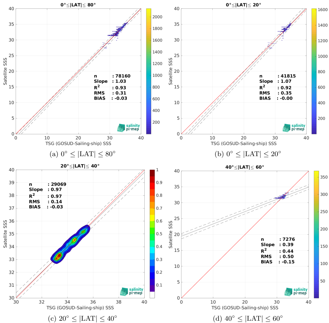
Figure 10: Contour maps of the concentration of CCI SSS L4 Merged-OI v5.5 - 7-day running (ESA) SSS (y-axis) versus TSG (GOSUD-Sailing-ship) SSS (x-axis) at match-up pairs for different latitude bands. For each plot, the red line shows x=y . The black thin and dashed lines indicate a linear fit through the data cloud and the \pm 95\% confidence levels, respectively. The number match-up pairs n , the slope and R^2 coefficient of the linear fit, the root mean square (RMS) and the mean bias between satellite and in situ data are indicated for each latitude band in each plots.
