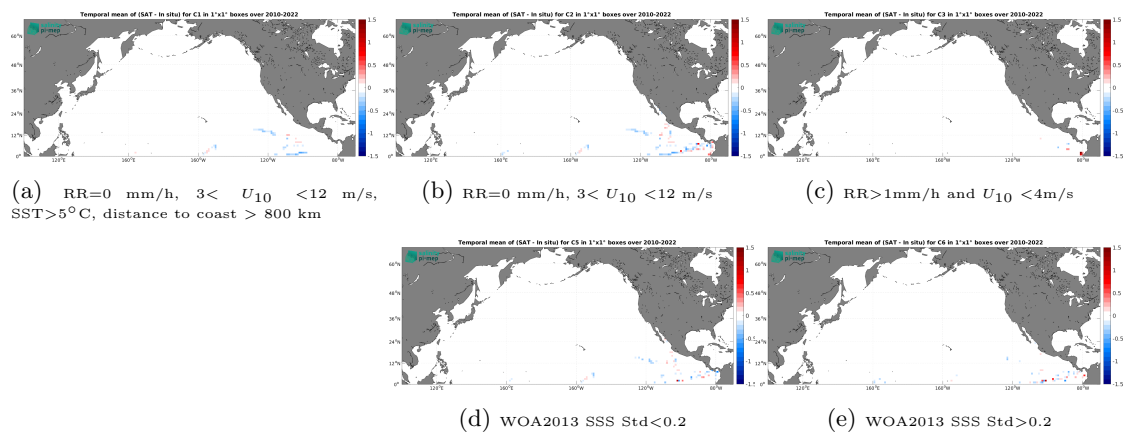
Figure 14: Temporal mean gridded over spatial boxes of size 1^\circ \times 1^\circ of \Delta\text{SSS} (CCI SSS L4 Merged-OI v5.5 - 7-day running (ESA) - TSG (GOSUD-Research-vessel)) for 5 different subdatasets corresponding to:RR=0 mm/h, 3 < U_{10} < 12 m/s, SST >5^\circ\text{C} , distance to coast > 800 km (a), RR=0 mm/h, 3 < U_{10} < 12 m/s (b), RR >1 mm/h and U_{10} < 4 m/s (c), WOA2013 SSS Std <0.2 (d), WOA2013 SSS Std >0.2 (e).
