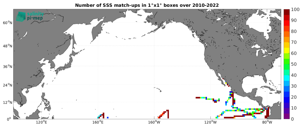
Figure 5: Number of SSS match-ups between TSG (GOSUD-Research-vessel) SSS and the CCI SSS L4 Merged-OI v5.5 - 7-day running (ESA) SSS product for the North Pacific Ocean Pi-MEP region over 1^\circ \times 1^\circ boxes and for the full satellite product period.
