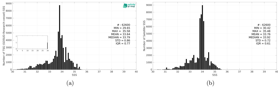
Figure 3: Histograms of SSS from TSG (GOSUD-Research-vessel) (a) and CCI SSS L4 Merged-OI v5.5 - 7-day running (ESA) (b) considering all match-up pairs per bins of 0.1 over the North Pacific Ocean Pi-MEP region and for the full satellite product period.
