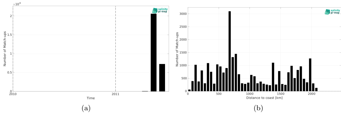
Figure 2: Number of match-ups between TSG (CSIC-UTM) and CCI SSS L4 Merged-OI v5.5 - 7-day running (ESA) SSS as a function of time (a) and as function of the distance to coast (b) over the North Pacific Ocean Pi-MEP region and for the full satellite product period.
