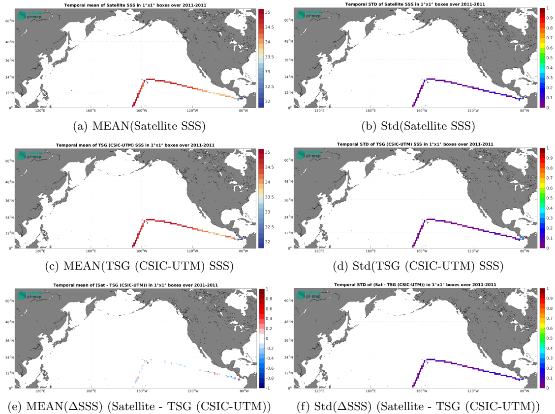
Figure 7: Temporal mean (left) and Std (right) of SSS from CCI SSS L4 Merged-OI v5.5 - 7-day running (ESA) (top), TSG (CSIC-UTM) ( in situ ) dataset (middle), and of \Delta SSS (Satellite - TSG (CSIC-UTM)). Only match-up pairs are used to generate these maps.
