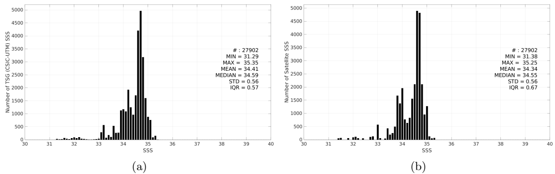
Figure 3: Histograms of SSS from TSG (CSIC-UTM) (a) and CCI SSS L4 Merged-OI v5.5 - 7-day running (ESA) (b) considering all match-up pairs per bins of 0.1 over the North Pacific Ocean Pi-MEP region and for the full satellite product period.
