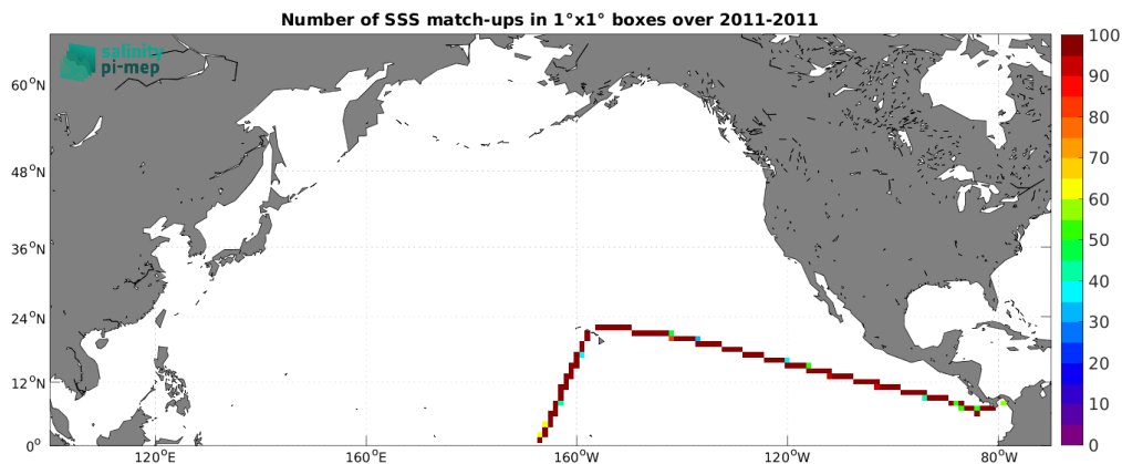
Figure 5: Number of SSS match-ups between TSG (CSIC-UTM) SSS and the CCI SSS L4 Merged-OI v5.5 - 7-day running (ESA) SSS product for the North Pacific Ocean Pi-MEP region over 1^\circ \times 1^\circ boxes and for the full satellite product period.
