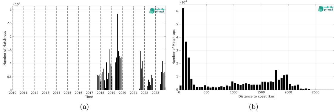
Figure 2: Number of match-ups between Saildrone and CCI SSS L4 Merged-OI v5.5 - 7-day running (ESA) SSS as a function of time (a) and as function of the distance to coast (b) over the North Pacific Ocean Pi-MEP region and for the full satellite product period.
