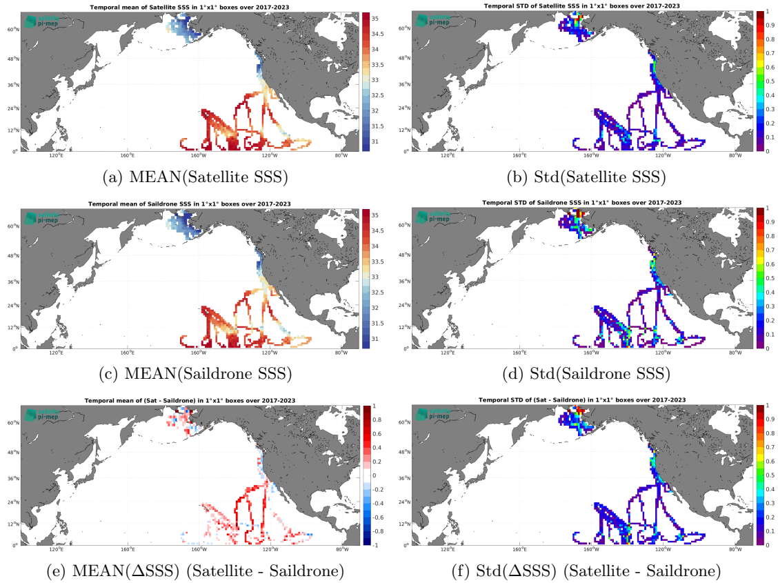
Figure 7: Temporal mean (left) and Std (right) of SSS from CCI SSS L4 Merged-OI v5.5 - 7-day running (ESA) (top), Saildrone (middle), and of \Delta SSS (Satellite - Saildrone). Only match-up pairs are used to generate these maps.
