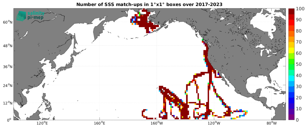
Figure 5: Number of SSS match-ups between Saildrone SSS and the CCI SSS L4 Merged-OI v5.5 - 7-day running (ESA) SSS product for the North Pacific Ocean Pi-MEP region over 1^\circ \times 1^\circ boxes and for the full satellite product period.
