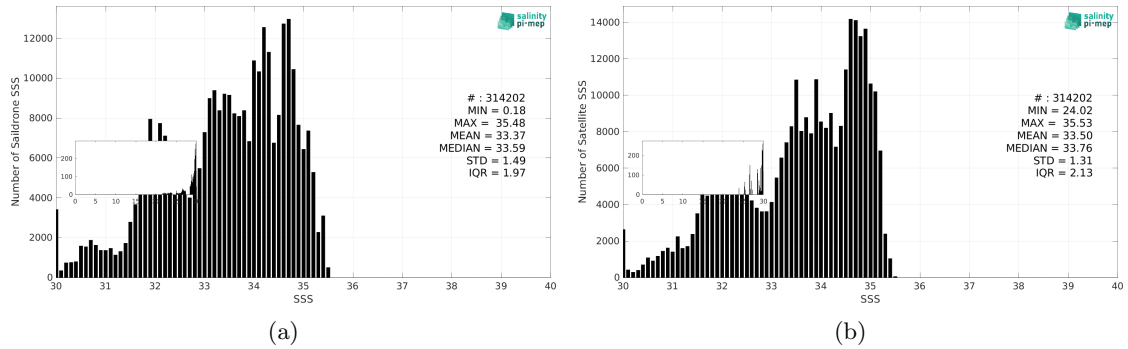
Figure 3: Histograms of SSS from Saildrone (a) and CCI SSS L4 Merged-OI v5.5 - 7-day running (ESA) (b) considering all match-up pairs per bins of 0.1 over the North Pacific Ocean Pi-MEP region and for the full satellite product period.
