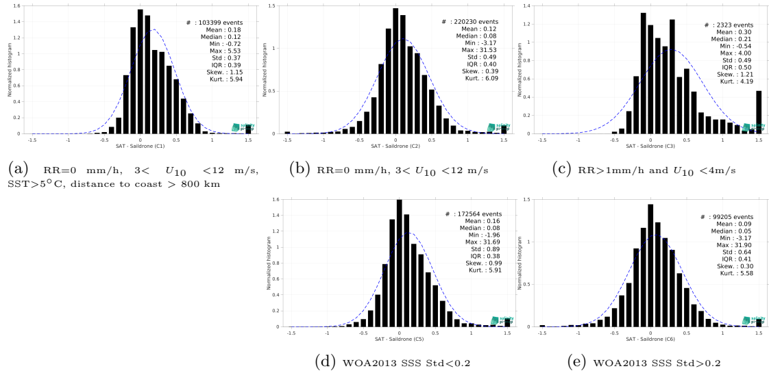
Figure 15: Normalized histogram of \Delta\text{SSS} (CCI SSS L4 Merged-OI v5.5 - 7-day running (ESA) - Sailldrone) for 5 different subdatasets corresponding to: RR=0 mm/h, 3 < U_{10} < 12 m/s, SST>5°C, distance to coast > 800 km (a), RR=0 mm/h, 3 < U_{10} < 12 m/s (b), RR>1mm/h and U_{10} < 4 m/s (c), WOA2013 SSS Std<0.2 (d), WOA2013 SSS Std>0.2 (e).
