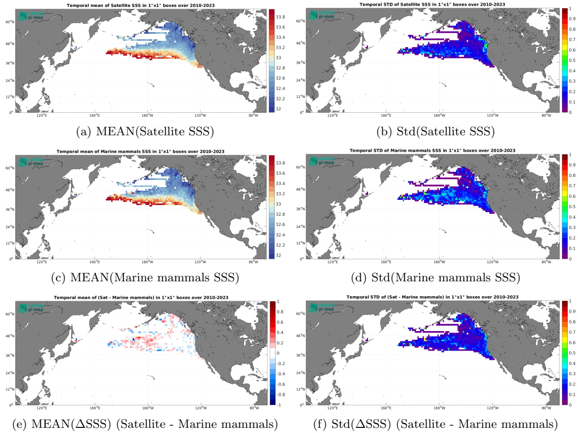
Figure 7: Temporal mean (left) and Std (right) of SSS from CCI SSS L4 Merged-OI v5.5 - 7-day running (ESA) (top), Marine mammals (middle), and of \Delta SSS (Satellite - Marine mammals). Only match-up pairs are used to generate these maps.
