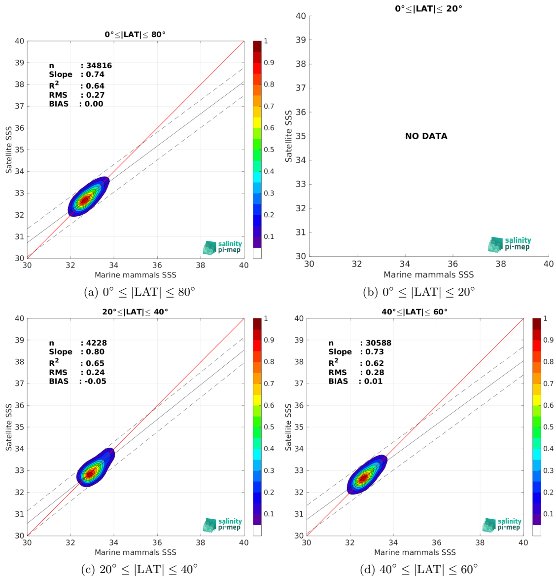
Figure 10: Contour maps of the concentration of CCI SSS L4 Merged-OI v5.5 - 7-day running (ESA) SSS (y-axis) versus Marine mammals SSS (x-axis) at match-up pairs for different latitude bands. For each plot, the red line shows x=y . The black thin and dashed lines indicate a linear fit through the data cloud and the \pm 95\% confidence levels, respectively. The number match-up pairs n , the slope and R^2 coefficient of the linear fit, the root mean square (RMS) and the mean bias between satellite and in situ data are indicated for each latitude band in each plots.
