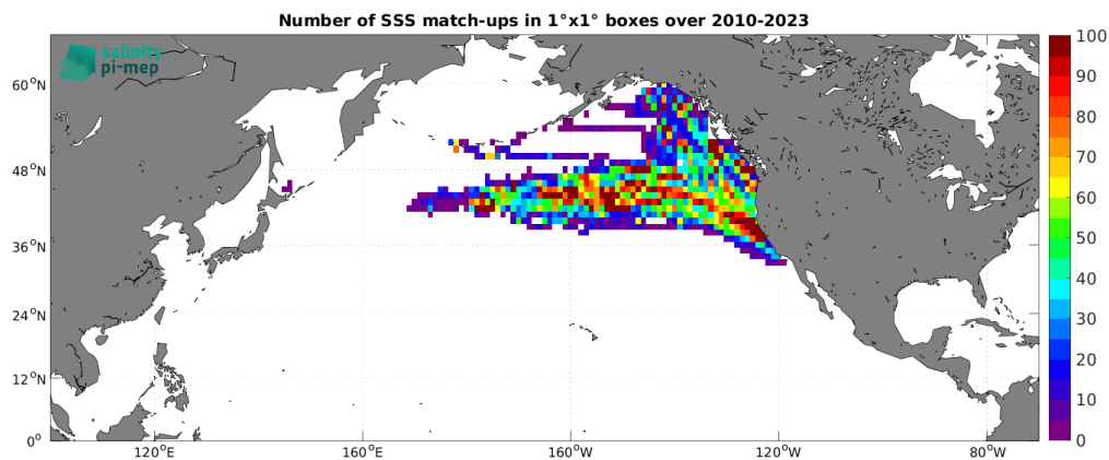
Figure 5: Number of SSS match-ups between Marine mammals SSS and the CCI SSS L4 Merged-OI v5.5 - 7-day running (ESA) SSS product for the North Pacific Ocean Pi-MEP region over 1^\circ \times 1^\circ boxes and for the full satellite product period.
