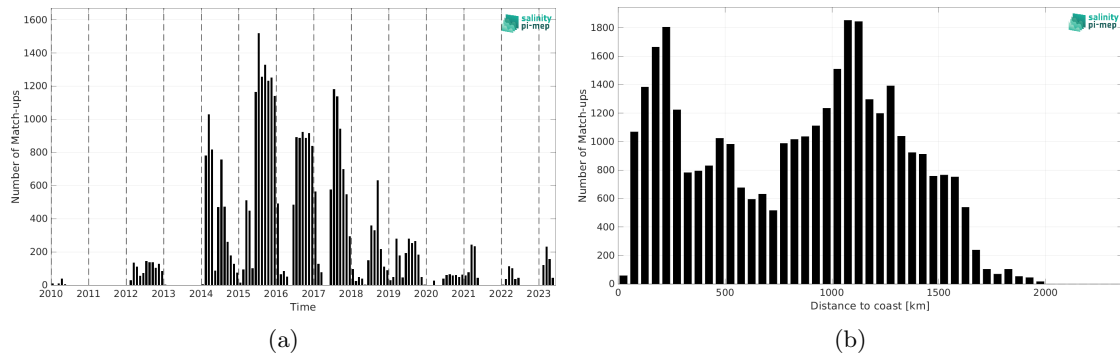
Figure 2: Number of match-ups between Marine mammals and CCI SSS L4 Merged-OI v5.5 - 7-day running (ESA) SSS as a function of time (a) and as function of the distance to coast (b) over the North Pacific Ocean Pi-MEP region and for the full satellite product period.
