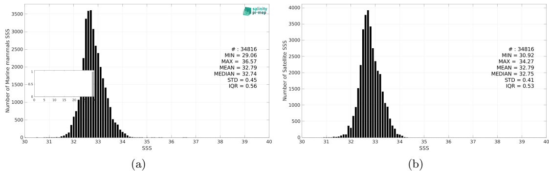
Figure 3: Histograms of SSS from Marine mammals (a) and CCI SSS L4 Merged-OI v5.5 - 7-day running (ESA) (b) considering all match-up pairs per bins of 0.1 over the North Pacific Ocean Pi-MEP region and for the full satellite product period.
