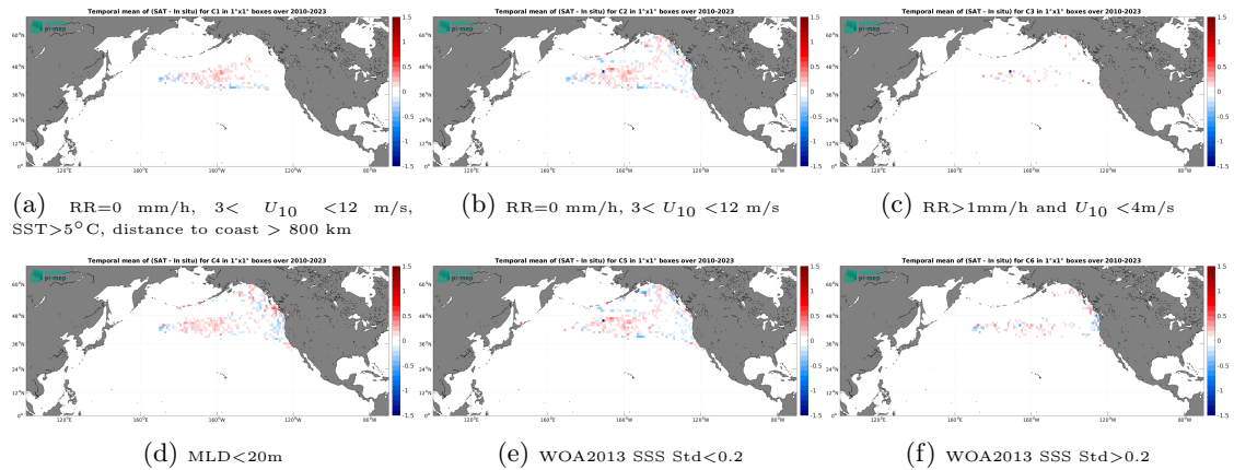
Figure 14: Temporal mean gridded over spatial boxes of size 1^\circ \times 1^\circ of \Delta SSS (CCI SSS L4 Merged-OI v5.5 - 7-day running (ESA) - Marine mammals) for 6 different subdatasets corresponding to:RR=0 mm/h, 3 < U_{10} < 12 m/s, SST >5^\circ C, distance to coast > 800 km (a), RR=0 mm/h, 3 < U_{10} < 12 m/s (b), RR >1 mm/h and U_{10} < 4 m/s (c),MLD <20 m (d),WOA2013 SSS Std <0.2 (e),WOA2013 SSS Std >0.2 (f).
