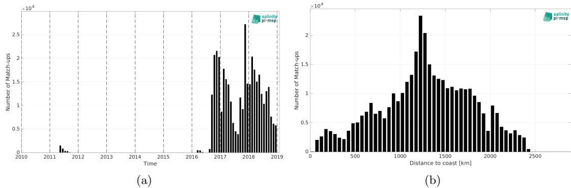
Figure 2: Number of match-ups between Surface drifters and CCI SSS L4 Merged-OI v5.5 - 7-day running (ESA) SSS as a function of time (a) and as function of the distance to coast (b) over the North Pacific Ocean Pi-MEP region and for the full satellite product period.
