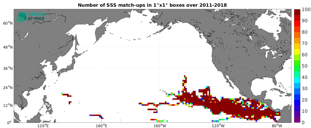
Figure 4: Number of SSS match-ups between Surface drifters SSS and the CCI SSS L4 Merged-OI v5.5 - 7-day running (ESA) SSS product for the North Pacific Ocean Pi-MEP region over 1^\circ \times 1^\circ boxes and for the full satellite product period.
