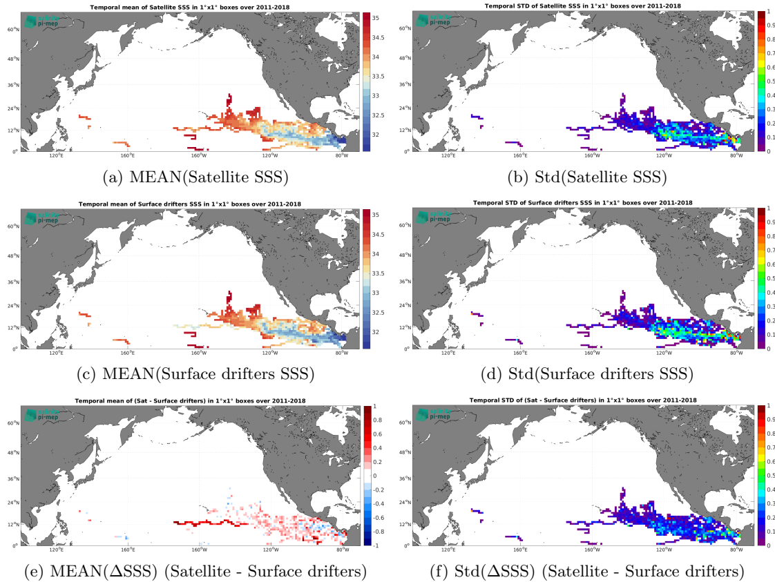
Figure 6: Temporal mean (left) and Std (right) of SSS from CCI SSS L4 Merged-OI v5.5 - 7-day running (ESA) (top), Surface drifters (middle), and of \Delta SSS (Satellite - Surface drifters). Only match-up pairs are used to generate these maps.
