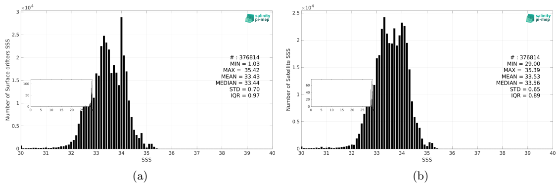
Figure 3: Histograms of SSS from Surface drifters (a) and CCI SSS L4 Merged-OI v5.5 - 7-day running (ESA) (b) considering all match-up pairs per bins of 0.1 over the North Pacific Ocean Pi-MEP region and for the full satellite product period.
