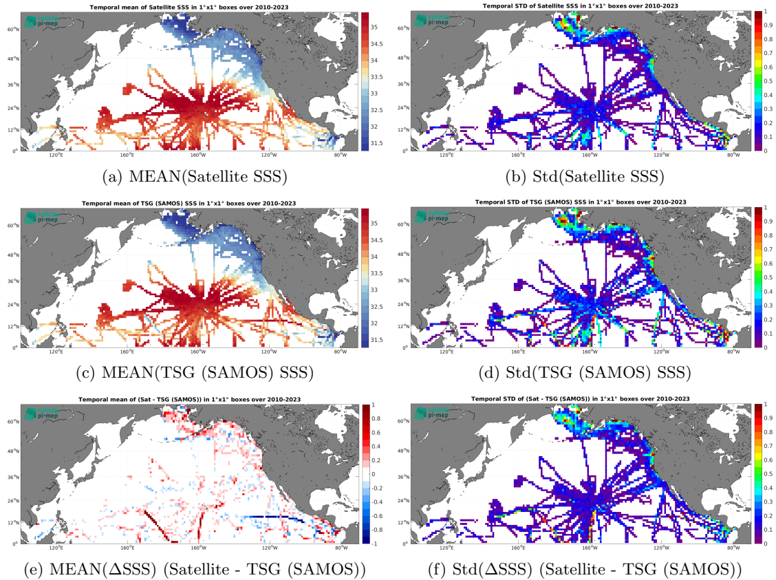
Figure 7: Temporal mean (left) and Std (right) of SSS from CCI SSS L4 Merged-OI v5.5 - 30-day running (ESA) (top), TSG (SAMOS) (middle), and of \Delta SSS (Satellite - TSG (SAMOS)). Only match-up pairs are used to generate these maps.
