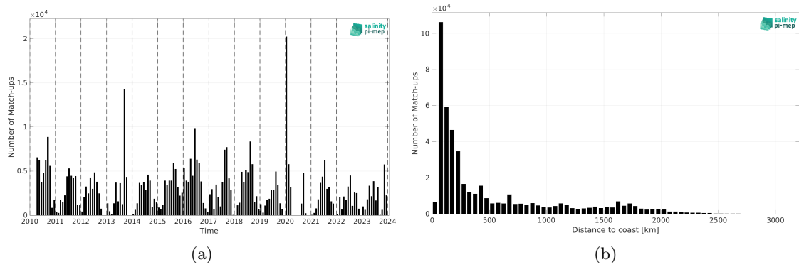
Figure 2: Number of match-ups between TSG (SAMOS) and CCI SSS L4 Merged-OI v5.5 - 30-day running (ESA) SSS as a function of time (a) and as function of the distance to coast (b) over the North Pacific Ocean Pi-MEP region and for the full satellite product period.
