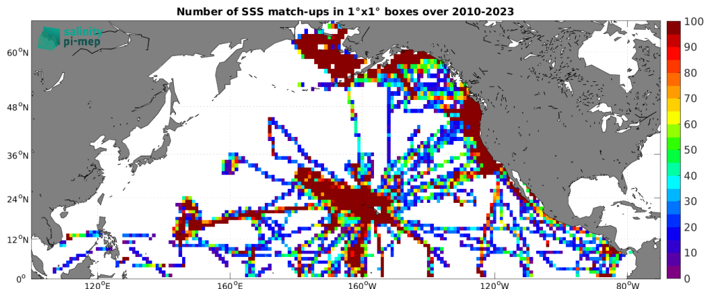
Figure 5: Number of SSS match-ups between TSG (SAMOS) SSS and the CCI SSS L4 Merged-OI v5.5 - 30-day running (ESA) SSS product for the North Pacific Ocean Pi-MEP region over 1^\circ \times 1^\circ boxes and for the full satellite product period.
