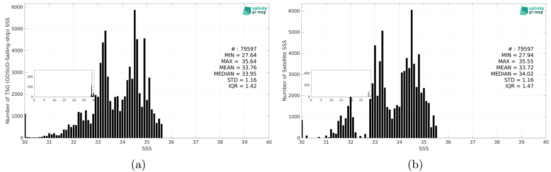
Figure 3: Histograms of SSS from TSG (GOSUD-Sailing-ship) (a) and CCI SSS L4 Merged-OI v5.5 - 30-day running (ESA) (b) considering all match-up pairs per bins of 0.1 over the North Pacific Ocean Pi-MEP region and for the full satellite product period.
