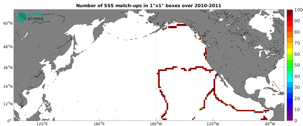
Figure 5: Number of SSS match-ups between TSG (GOSUD-Sailing-ship) SSS and the CCI SSS L4 Merged-OI v5.5 - 30-day running (ESA) SSS product for the North Pacific Ocean Pi-MEP region over 1^\circ \times 1^\circ boxes and for the full satellite product period.
