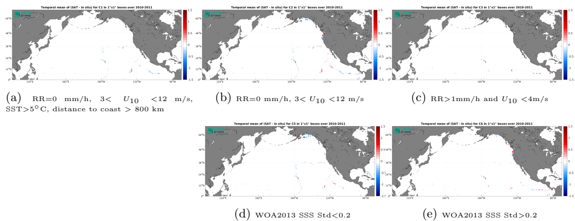
Figure 14: Temporal mean gridded over spatial boxes of size 1^\circ \times 1^\circ of \Delta SSS (CCI SSS L4 Merged-OI v5.5 - 30-day running (ESA) - TSG (GOSUD-Sailing-ship)) for 5 different subdatasets corresponding to:RR=0 mm/h, 3 < U_{10} < 12 m/s, SST >5^\circ\text{C} , distance to coast > 800 km (a), RR=0 mm/h, 3 < U_{10} < 12 m/s (b), RR >1 mm/h and U_{10} < 4 m/s (c), WOA2013 SSS Std <0.2 (d), WOA2013 SSS Std >0.2 (e).
