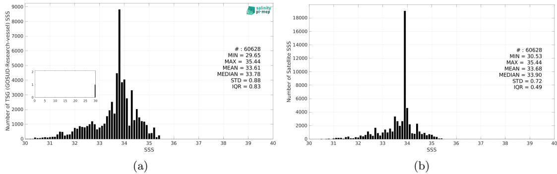
Figure 3: Histograms of SSS from TSG (GOSUD-Research-vessel) (a) and CCI SSS L4 Merged-OI v5.5 - 30-day running (ESA) (b) considering all match-up pairs per bins of 0.1 over the North Pacific Ocean Pi-MEP region and for the full satellite product period.
