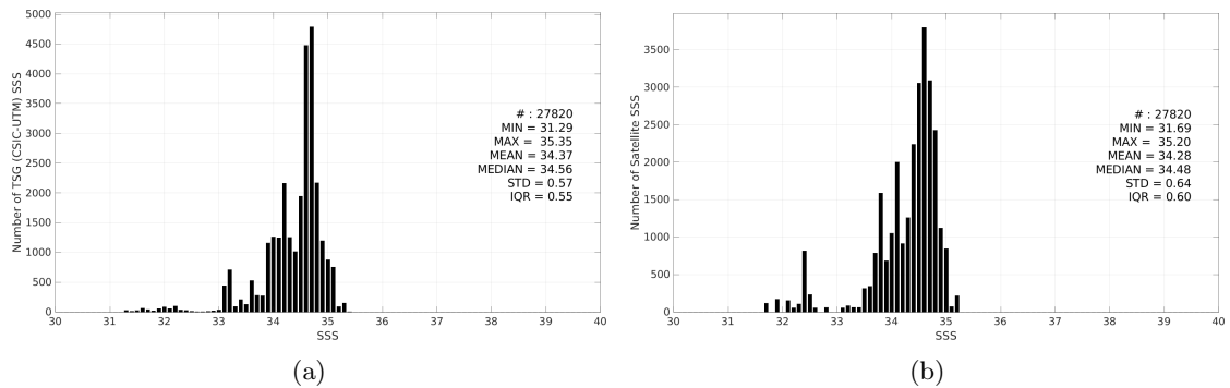
Figure 3: Histograms of SSS from TSG (CSIC-UTM) (a) and CCI SSS L4 Merged-OI v5.5 - 30-day running (ESA) (b) considering all match-up pairs per bins of 0.1 over the North Pacific Ocean Pi-MEP region and for the full satellite product period.
