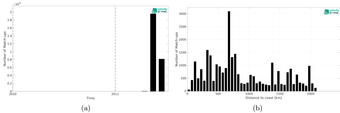
Figure 2: Number of match-ups between TSG (CSIC-UTM) and CCI SSS L4 Merged-OI v5.5 - 30-day running (ESA) SSS as a function of time (a) and as function of the distance to coast (b) over the North Pacific Ocean Pi-MEP region and for the full satellite product period.
