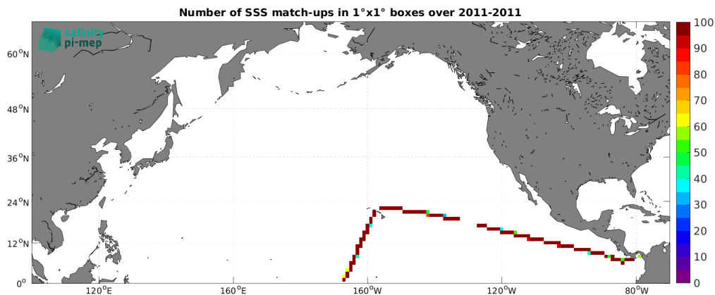
Figure 5: Number of SSS match-ups between TSG (CSIC-UTM) SSS and the CCI SSS L4 Merged-OI v5.5 - 30-day running (ESA) SSS product for the North Pacific Ocean Pi-MEP region over 1^\circ \times 1^\circ boxes and for the full satellite product period.
