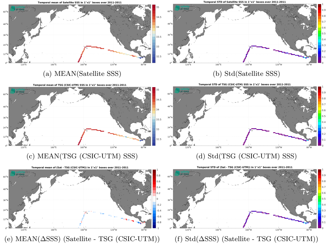
Figure 7: Temporal mean (left) and Std (right) of SSS from CCI SSS L4 Merged-OI v5.5 - 30-day running (ESA) (top), TSG (CSIC-UTM) (middle), and of \Delta SSS (Satellite - TSG (CSIC-UTM)). Only match-up pairs are used to generate these maps.
