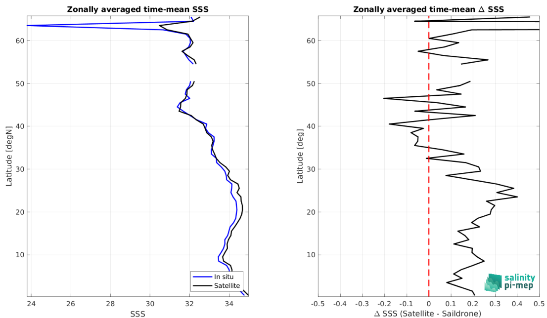
Figure 9: Left panel: Zonal mean SSS from CCI SSS L4 Merged-OI v5.5 - 30-day running (ESA) satellite product (black) and from Saildrone (blue). Right panel: Zonal mean of \Delta SSS (Satellite - Saildrone) for all the collected Pi-MEP match-up pairs estimated over the full satellite product period.
