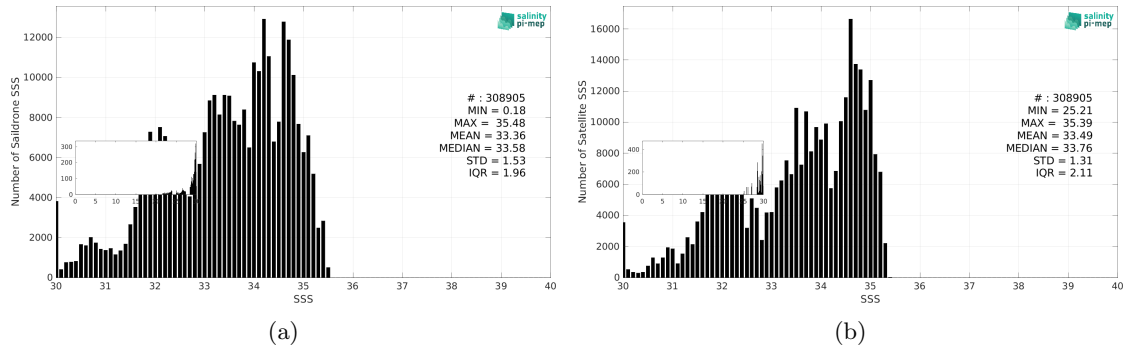
Figure 3: Histograms of SSS from Saildrone (a) and CCI SSS L4 Merged-OI v5.5 - 30-day running (ESA) (b) considering all match-up pairs per bins of 0.1 over the North Pacific Ocean Pi-MEP region and for the full satellite product period.
