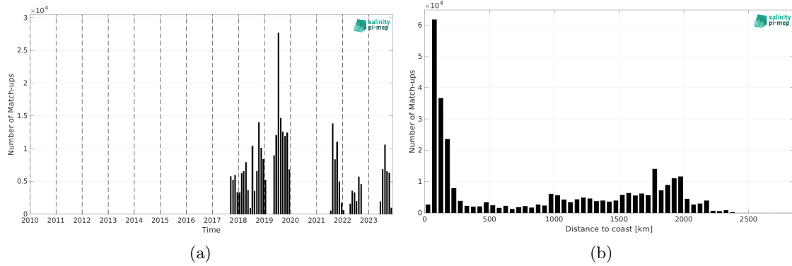
Figure 2: Number of match-ups between Saildrone and CCI SSS L4 Merged-OI v5.5 - 30-day running (ESA) SSS as a function of time (a) and as function of the distance to coast (b) over the North Pacific Ocean Pi-MEP region and for the full satellite product period.
