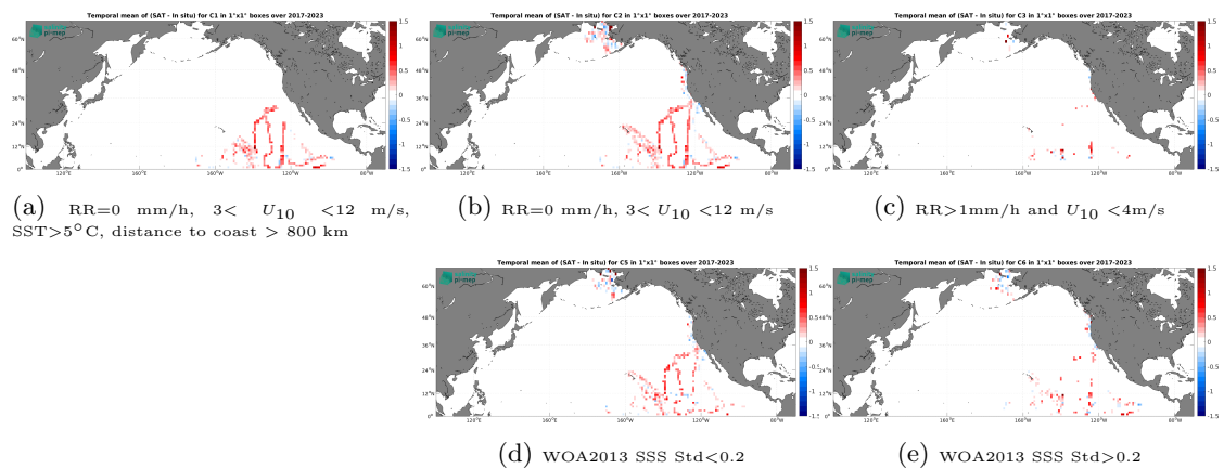
Figure 14: Temporal mean gridded over spatial boxes of size 1^\circ \times 1^\circ of \Delta SSS (CCI SSS L4 Merged-OI v5.5 - 30-day running (ESA) - Saildrone) for 5 different subdatasets corresponding to:RR=0 mm/h, 3 < U_{10} < 12 m/s, SST>5°C, distance to coast > 800 km (a), RR=0 mm/h, 3 < U_{10} < 12 m/s (b), RR>1mm/h and U_{10} < 4 m/s (c), WOA2013 SSS Std<0.2 (d), WOA2013 SSS Std>0.2 (e).
