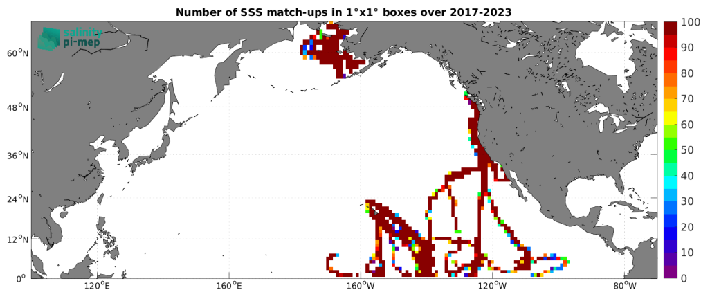
Figure 5: Number of SSS match-ups between Saildrone SSS and the CCI SSS L4 Merged-OI v5.5 - 30-day running (ESA) SSS product for the North Pacific Ocean Pi-MEP region over 1^\circ \times 1^\circ boxes and for the full satellite product period.
