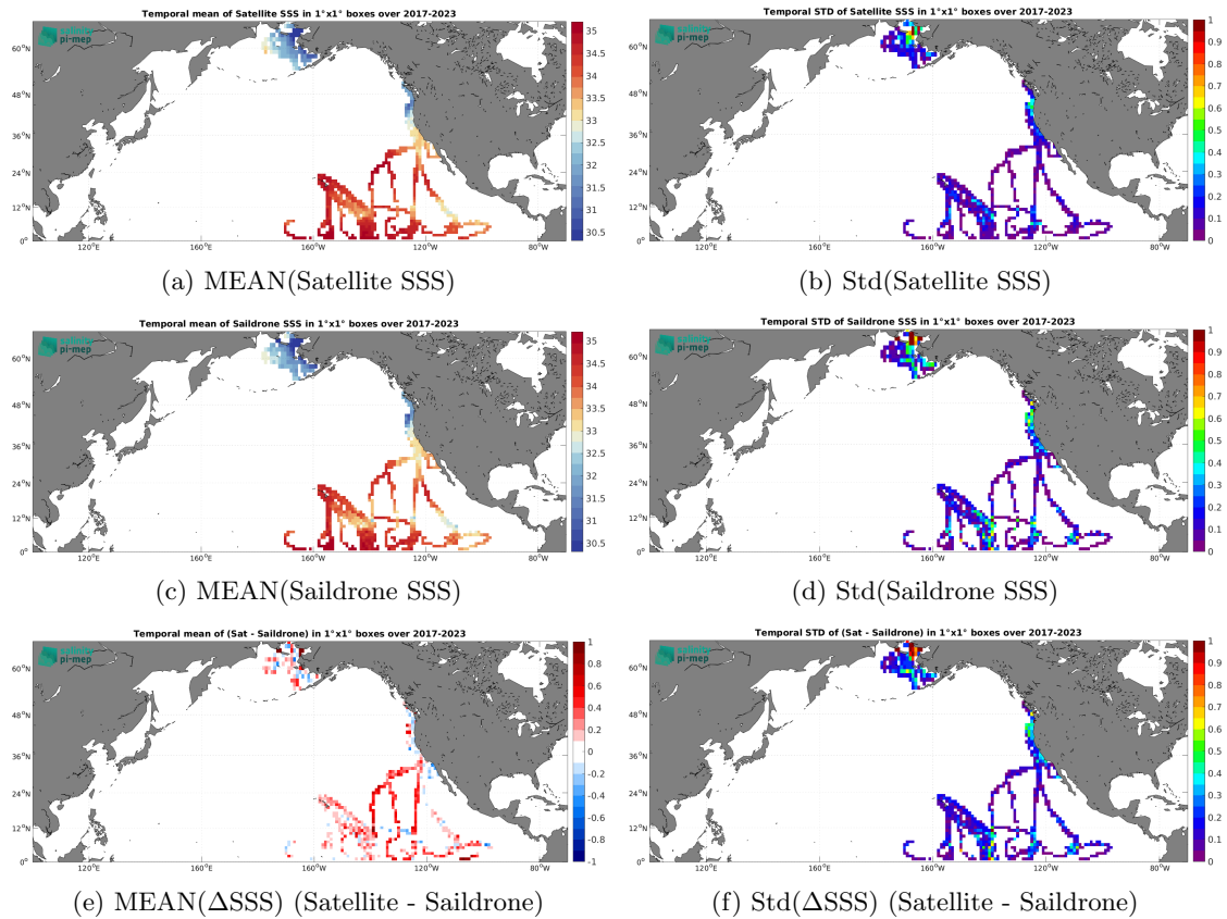
Figure 7: Temporal mean (left) and Std (right) of SSS from CCI SSS L4 Merged-OI v5.5 - 30-day running (ESA) (top), Saildrone (middle), and of \Delta SSS (Satellite - Saildrone). Only match-up pairs are used to generate these maps.
