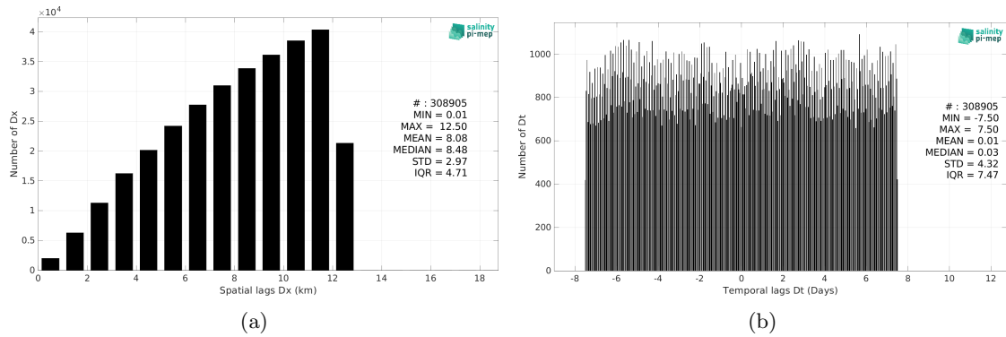
Figure 6: Histograms of the spatial (a) and temporal (b) lags between the location/time of the Saildrone measurement and the date of the corresponding CCI SSS L4 Merged-OI v5.5 - 30-day running (ESA) SSS pixel.
