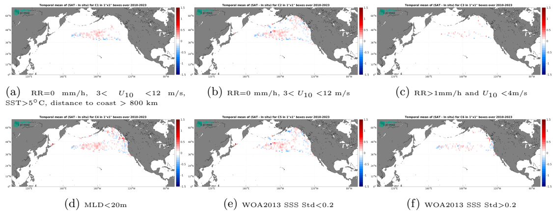
Figure 14: Temporal mean gridded over spatial boxes of size 1^\circ \times 1^\circ of \Delta SSS (CCI SSS L4 Merged-OI v5.5 - 30-day running (ESA) - Marine mammals) for 6 different subdatasets corresponding to:RR=0 mm/h, 3 < U_{10} < 12 m/s, SST >5^\circ C, distance to coast > 800 km (a), RR=0 mm/h, 3 < U_{10} < 12 m/s (b), RR >1 mm/h and U_{10} < 4 m/s (c),MLD <20 m (d),WOA2013 SSS Std <0.2 (e),WOA2013 SSS Std >0.2 (f).
