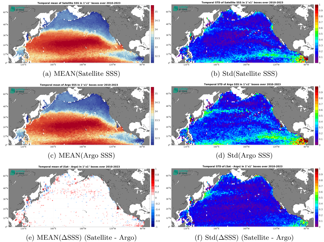
Figure 7: Temporal mean (left) and Std (right) of SSS from CCI SSS L4 Merged-OI v5.5 - 30-day running (ESA) (top), Argo (middle), and of \Delta SSS (Satellite - Argo). Only match-up pairs are used to generate these maps.
