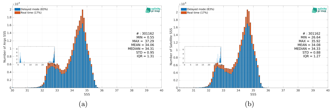
Figure 3: Histograms of SSS from Argo (a) and CCI SSS L4 Merged-OI v5.5 - 30-day running (ESA) (b) considering all match-up pairs per bins of 0.1 over the North Pacific Ocean Pi-MEP region and for the full satellite product period.
