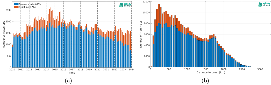
Figure 2: Number of match-ups between Argo and CCI SSS L4 Merged-OI v5.5 - 30-day running (ESA) SSS as a function of time (a) and as function of the distance to coast (b) over the North Pacific Ocean Pi-MEP region and for the full satellite product period.
