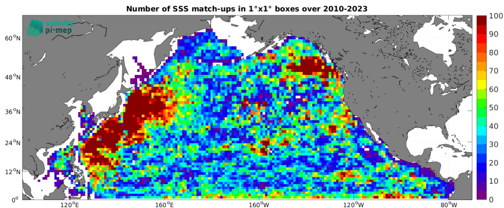
Figure 5: Number of SSS match-ups between Argo SSS and the CCI SSS L4 Merged-OI v5.5 - 30-day running (ESA) SSS product for the North Pacific Ocean Pi-MEP region over 1^\circ \times 1^\circ boxes and for the full satellite product period.
