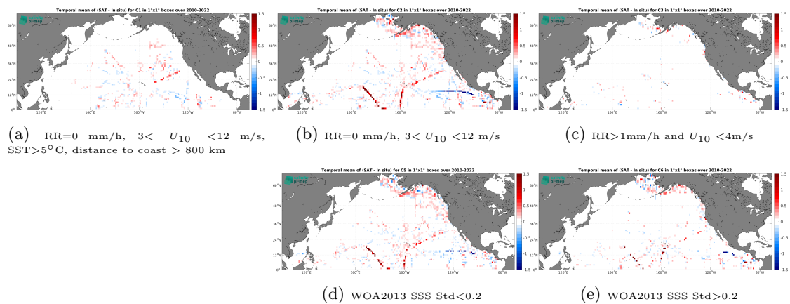
Figure 14: Temporal mean gridded over spatial boxes of size 1^\circ \times 1^\circ of \Delta\text{SSS} (CCI SSS L4 Merged-OI v4.41 - 7-day running (ESA) - TSG (SAMOS)) for 5 different subdatasets corresponding to:RR=0 mm/h, 3 < U_{10} < 12 m/s, SST>5°C, distance to coast > 800 km (a), RR=0 mm/h, 3 < U_{10} < 12 m/s (b), RR>1mm/h and U_{10} < 4 m/s (c), WOA2013 SSS Std<0.2 (d), WOA2013 SSS Std>0.2 (e).
