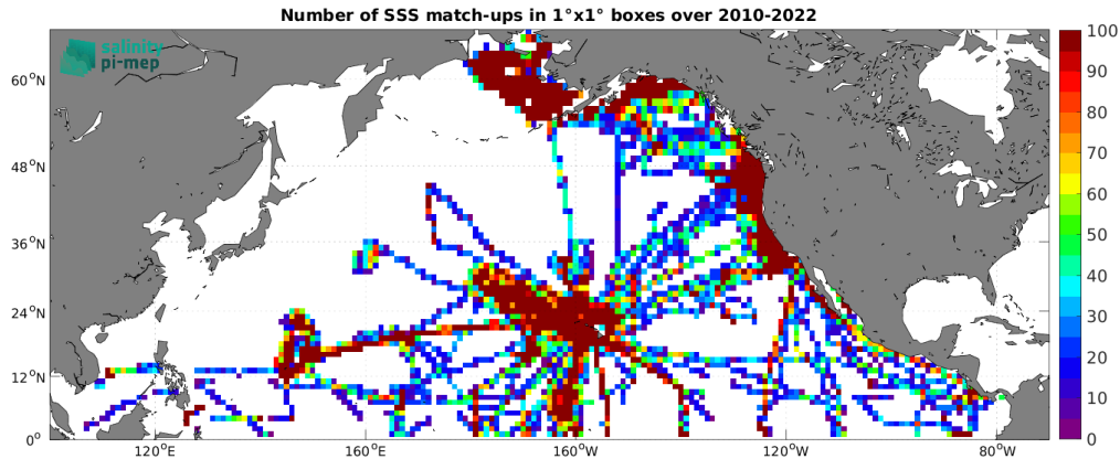
Figure 5: Number of SSS match-ups between TSG (SAMOS) SSS and the CCI SSS L4 Merged-OI v4.41 - 7-day running (ESA) SSS product for the North Pacific Ocean Pi-MEP region over 1^\circ \times 1^\circ boxes and for the full satellite product period.
