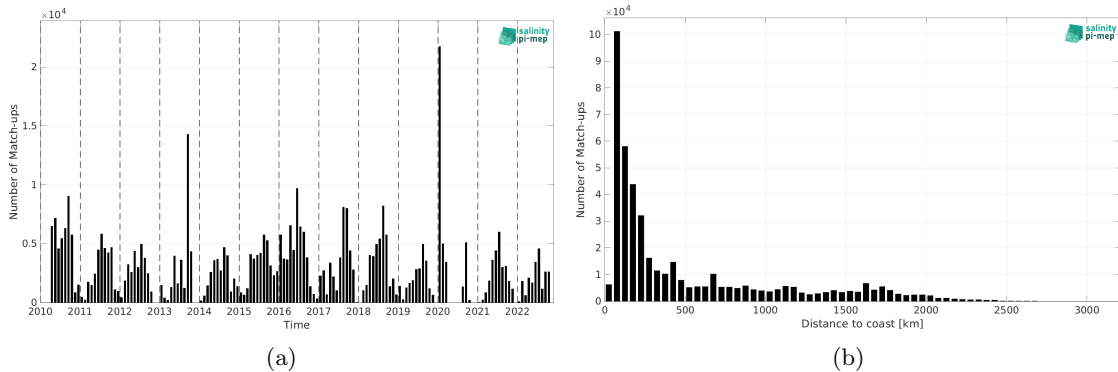
Figure 2: Number of match-ups between TSG (SAMOS) and CCI SSS L4 Merged-OI v4.41 - 7-day running (ESA) SSS as a function of time (a) and as function of the distance to coast (b) over the North Pacific Ocean Pi-MEP region and for the full satellite product period.
