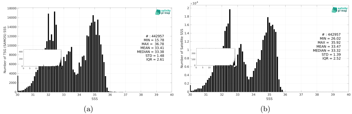
Figure 3: Histograms of SSS from TSG (SAMOS) (a) and CCI SSS L4 Merged-OI v4.41 - 7-day running (ESA) (b) considering all match-up pairs per bins of 0.1 over the North Pacific Ocean Pi-MEP region and for the full satellite product period.
