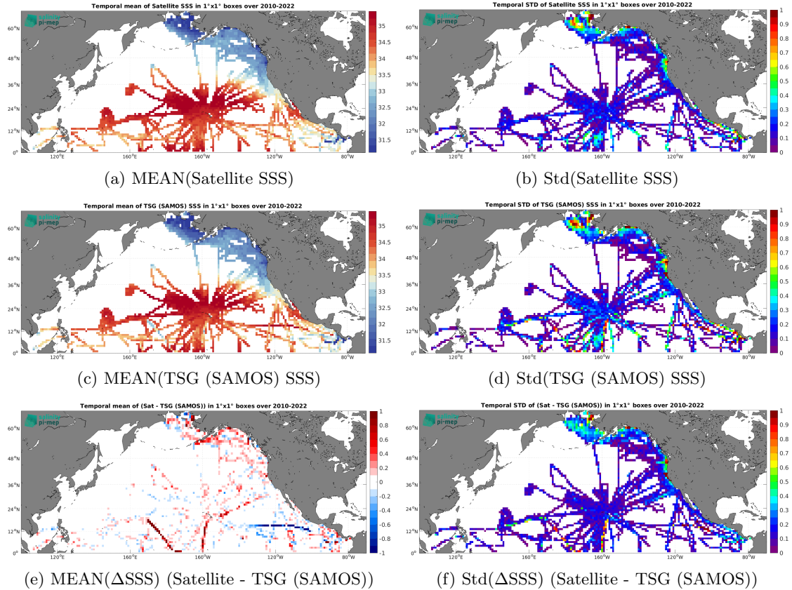
Figure 7: Temporal mean (left) and Std (right) of SSS from CCI SSS L4 Merged-OI v4.41 - 7-day running (ESA) (top), TSG (SAMOS) (middle), and of \Delta\text{SSS} (Satellite - TSG (SAMOS)). Only match-up pairs are used to generate these maps.
