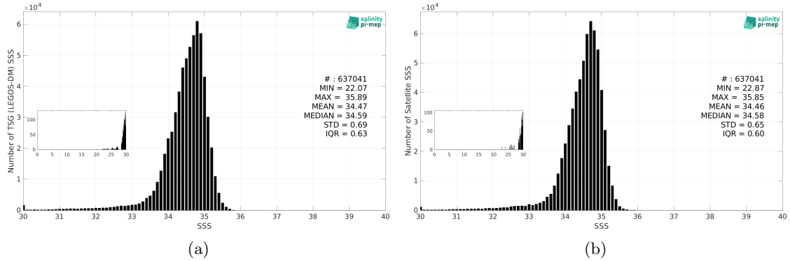
Figure 3: Histograms of SSS from TSG (LEGOS-DM) (a) and CCI SSS L4 Merged-OI v4.41 - 7-day running (ESA) (b) considering all match-up pairs per bins of 0.1 over the North Pacific Ocean Pi-MEP region and for the full satellite product period.
