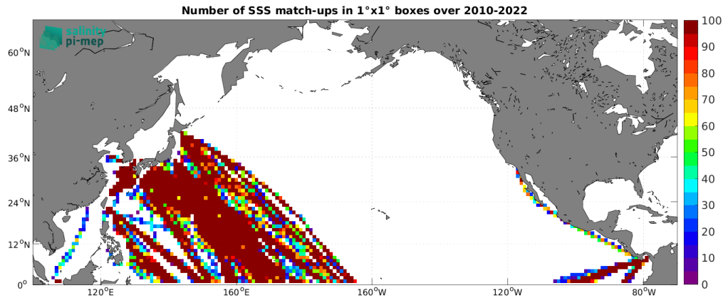
Figure 5: Number of SSS match-ups between TSG (LEGOS-DM) SSS and the CCI SSS L4 Merged-OI v4.41 - 7-day running (ESA) SSS product for the North Pacific Ocean Pi-MEP region over 1^\circ \times 1^\circ boxes and for the full satellite product period.
