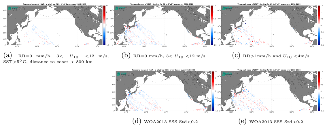
Figure 14: Temporal mean gridded over spatial boxes of size 1^\circ \times 1^\circ of \Delta SSS (CCI SSS L4 Merged-OI v4.41 - 7-day running (ESA) - TSG (LEGOS-DM)) for 5 different subdatasets corresponding to:RR=0 mm/h, 3 < U_{10} < 12 m/s, SST>5°C, distance to coast > 800 km (a), RR=0 mm/h, 3 < U_{10} < 12 m/s (b), RR>1mm/h and U_{10} < 4 m/s (c), WOA2013 SSS Std<0.2 (d), WOA2013 SSS Std>0.2 (e).
