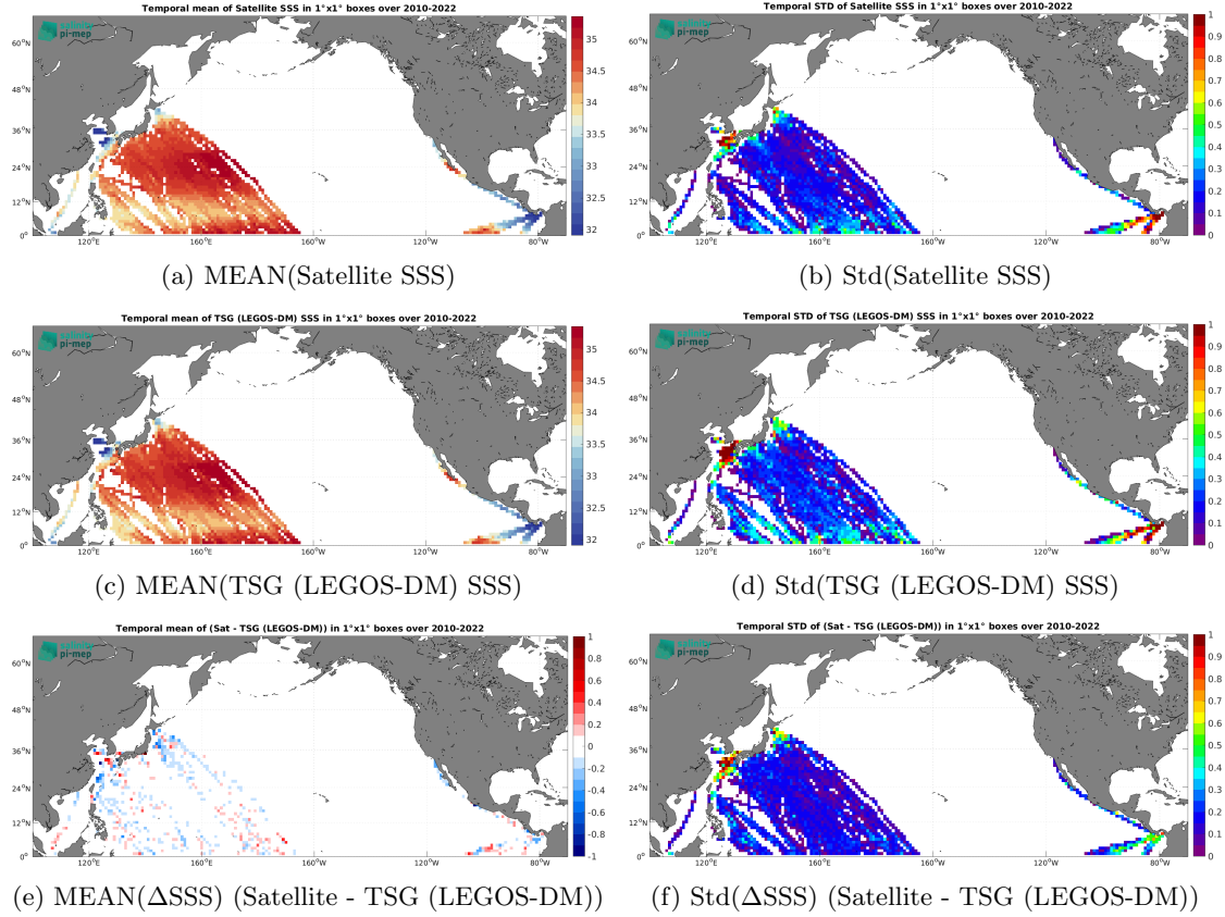
Figure 7: Temporal mean (left) and Std (right) of SSS from CCI SSS L4 Merged-OI v4.41 - 7-day running (ESA) (top), TSG (LEGOS-DM) (middle), and of \Delta\text{SSS} (Satellite - TSG (LEGOS-DM)). Only match-up pairs are used to generate these maps.
