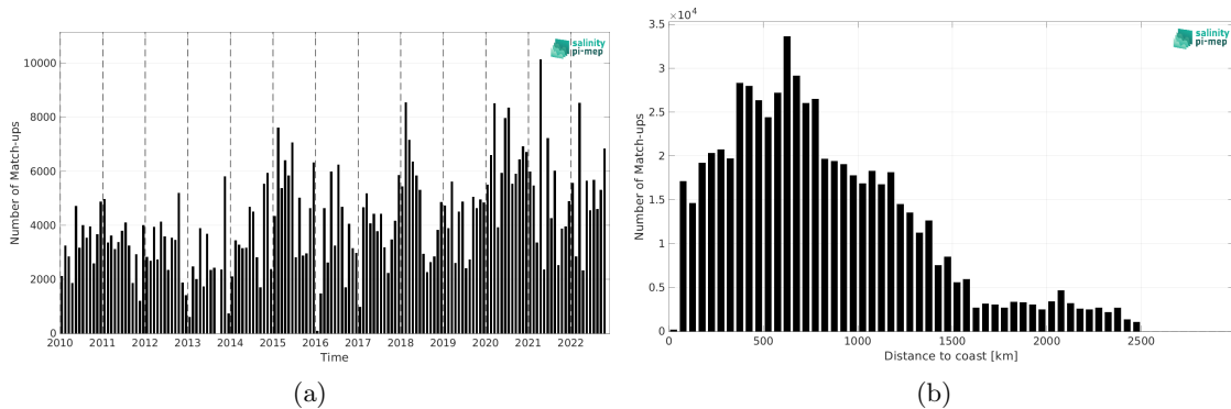
Figure 2: Number of match-ups between TSG (LEGOS-DM) and CCI SSS L4 Merged-OI v4.41 - 7-day running (ESA) SSS as a function of time (a) and as function of the distance to coast (b) over the North Pacific Ocean Pi-MEP region and for the full satellite product period.
