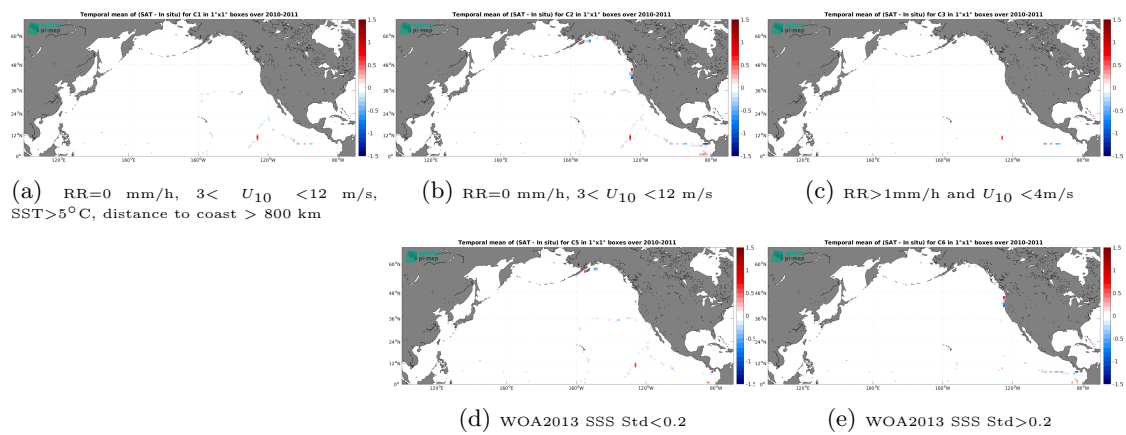
Figure 14: Temporal mean gridded over spatial boxes of size 1^\circ \times 1^\circ of \Delta SSS (CCI SSS L4 Merged-OI v4.41 - 7-day running (ESA) - TSG (GOSUD-Sailing-ship)) for 5 different subdatasets corresponding to:RR=0 mm/h, 3 < U_{10} < 12 m/s, SST >5^\circ\text{C} , distance to coast > 800 km (a), RR=0 mm/h, 3 < U_{10} < 12 m/s (b), RR >1 mm/h and U_{10} < 4 m/s (c), WOA2013 SSS Std <0.2 (d), WOA2013 SSS Std >0.2 (e).
