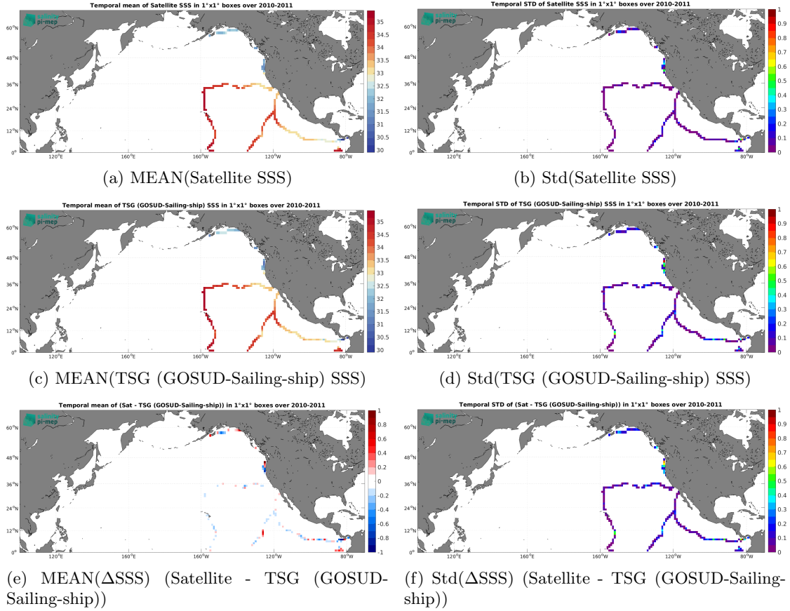
Figure 7: Temporal mean (left) and Std (right) of SSS from CCI SSS L4 Merged-OI v4.41 - 7-day running (ESA) (top), TSG (GOSUD-Sailing-ship) (middle), and of \Delta SSS (Satellite - TSG (GOSUD-Sailing-ship)). Only match-up pairs are used to generate these maps.
