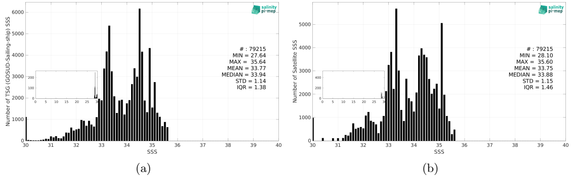
Figure 3: Histograms of SSS from TSG (GOSUD-Sailing-ship) (a) and CCI SSS L4 Merged-OI v4.41 - 7-day running (ESA) (b) considering all match-up pairs per bins of 0.1 over the North Pacific Ocean Pi-MEP region and for the full satellite product period.
