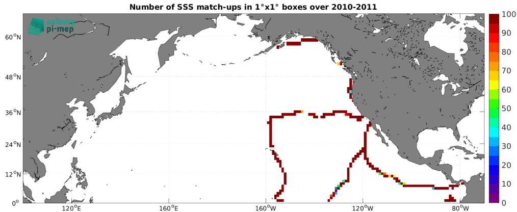
Figure 5: Number of SSS match-ups between TSG (GOSUD-Sailing-ship) SSS and the CCI SSS L4 Merged-OI v4.41 - 7-day running (ESA) SSS product for the North Pacific Ocean Pi-MEP region over 1^\circ \times 1^\circ boxes and for the full satellite product period.
