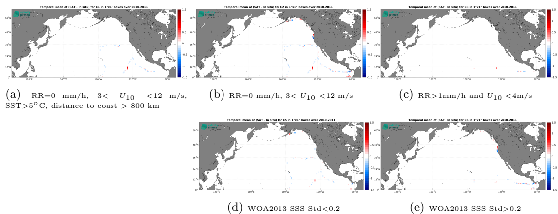
Figure 14: Temporal mean gridded over spatial boxes of size 1^\circ \times 1^\circ of \Delta\text{SSS} (CCI SSS L4 Merged-OI v4.41 - 7-day running (ESA) - TSG (GOSUD-Sailing-ship)) for 5 different subdatasets corresponding to: RR=0 mm/h, 3 < U_{10} < 12 m/s, SST > 5^\circ\text{C} , distance to coast > 800 km (a), RR=0 mm/h, 3 < U_{10} < 12 m/s (b), RR > 1 mm/h and U_{10} < 4 m/s (c), WOA2013 SSS Std < 0.2 (d), WOA2013 SSS Std > 0.2 (e).
