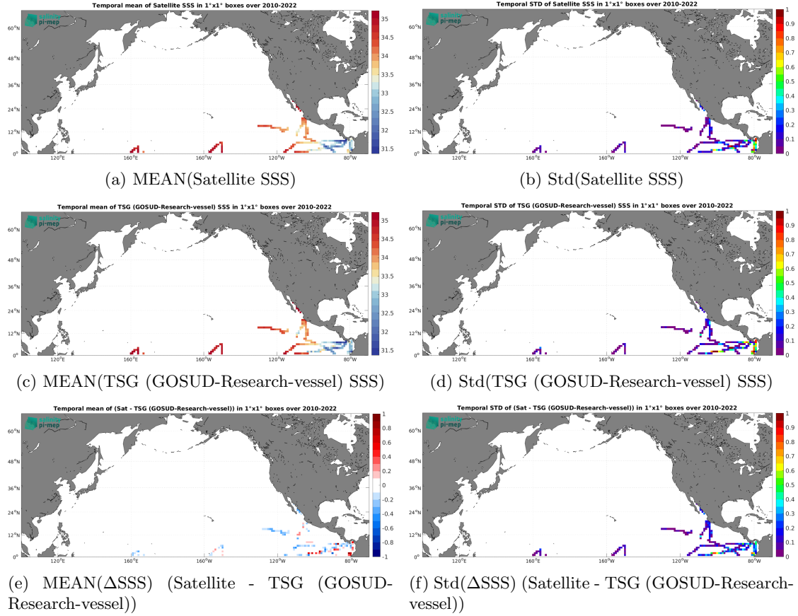
Figure 7: Temporal mean (left) and Std (right) of SSS from CCI SSS L4 Merged-OI v4.41 - 7-day running (ESA) (top), TSG (GOSUD-Research-vessel) (middle), and of \Delta SSS (Satellite - TSG (GOSUD-Research-vessel)). Only match-up pairs are used to generate these maps.
