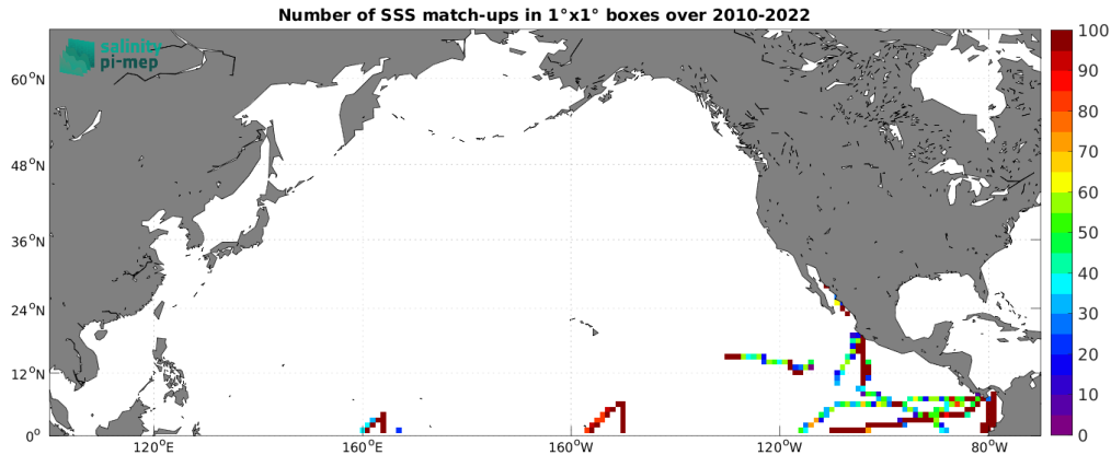
Figure 5: Number of SSS match-ups between TSG (GOSUD-Research-vessel) SSS and the CCI SSS L4 Merged-OI v4.41 - 7-day running (ESA) SSS product for the North Pacific Ocean Pi-MEP region over 1^\circ \times 1^\circ boxes and for the full satellite product period.
