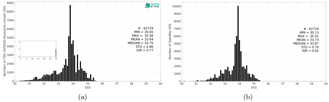
Figure 3: Histograms of SSS from TSG (GOSUD-Research-vessel) (a) and CCI SSS L4 Merged-OI v4.41 - 7-day running (ESA) (b) considering all match-up pairs per bins of 0.1 over the North Pacific Ocean Pi-MEP region and for the full satellite product period.
