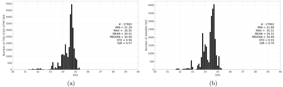
Figure 3: Histograms of SSS from TSG (CSIC-UTM) (a) and CCI SSS L4 Merged-OI v4.41 - 7-day running (ESA) (b) considering all match-up pairs per bins of 0.1 over the North Pacific Ocean Pi-MEP region and for the full satellite product period.
