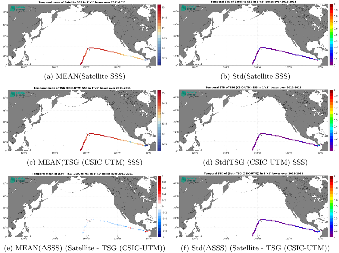
Figure 7: Temporal mean (left) and Std (right) of SSS from CCI SSS L4 Merged-OI v4.41 - 7-day running (ESA) (top), TSG (CSIC-UTM) (middle), and of \Delta SSS (Satellite - TSG (CSIC-UTM)). Only match-up pairs are used to generate these maps.
