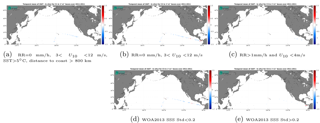
Figure 14: Temporal mean gridded over spatial boxes of size 1^\circ \times 1^\circ of \Delta\text{SSS} (CCI SSS L4 Merged-OI v4.41 - 7-day running (ESA) - TSG (CSIC-UTM)) for 5 different subdatasets corresponding to:RR=0 mm/h, 3 < U_{10} < 12 m/s, SST>5°C, distance to coast > 800 km (a), RR=0 mm/h, 3 < U_{10} < 12 m/s (b), RR>1mm/h and U_{10} < 4 m/s (c), WOA2013 SSS Std<0.2 (d), WOA2013 SSS Std>0.2 (e).
