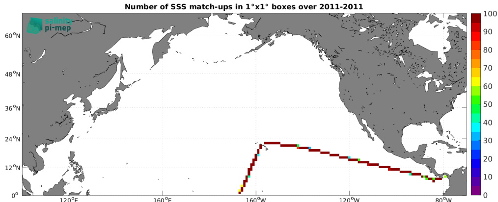
Figure 5: Number of SSS match-ups between TSG (CSIC-UTM) SSS and the CCI SSS L4 Merged-OI v4.41 - 7-day running (ESA) SSS product for the North Pacific Ocean Pi-MEP region over 1^\circ \times 1^\circ boxes and for the full satellite product period.
