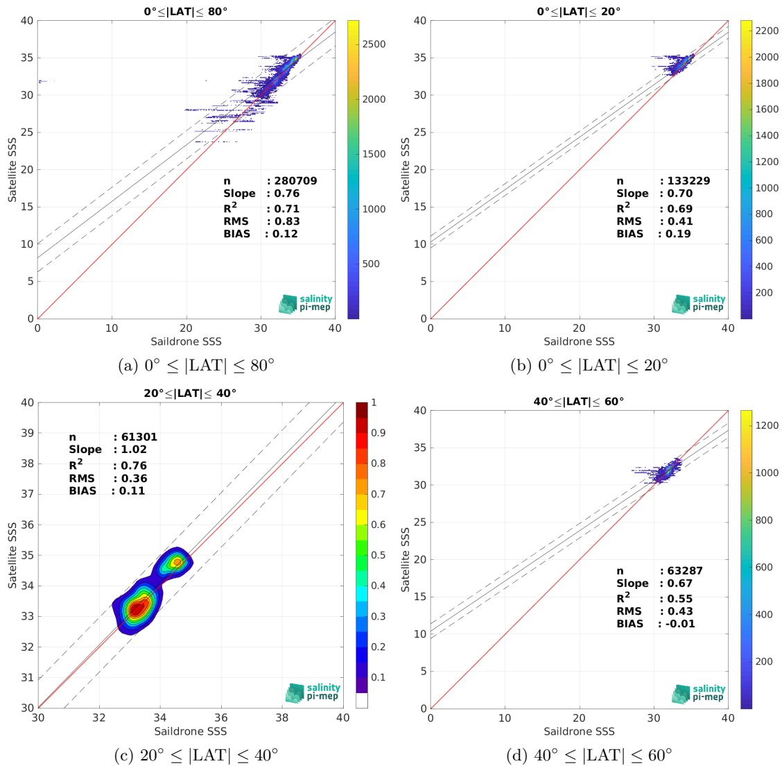
Figure 10: Contour maps of the concentration of CCI SSS L4 Merged-OI v4.41 - 7-day running (ESA) SSS (y-axis) versus Saildrone SSS (x-axis) at match-up pairs for different latitude bands. For each plot, the red line shows x=y . The black thin and dashed lines indicate a linear fit through the data cloud and the \pm 95\% confidence levels, respectively. The number match-up pairs n , the slope and R^2 coefficient of the linear fit, the root mean square (RMS) and the mean bias between satellite and in situ data are indicated for each latitude band in each plots.
