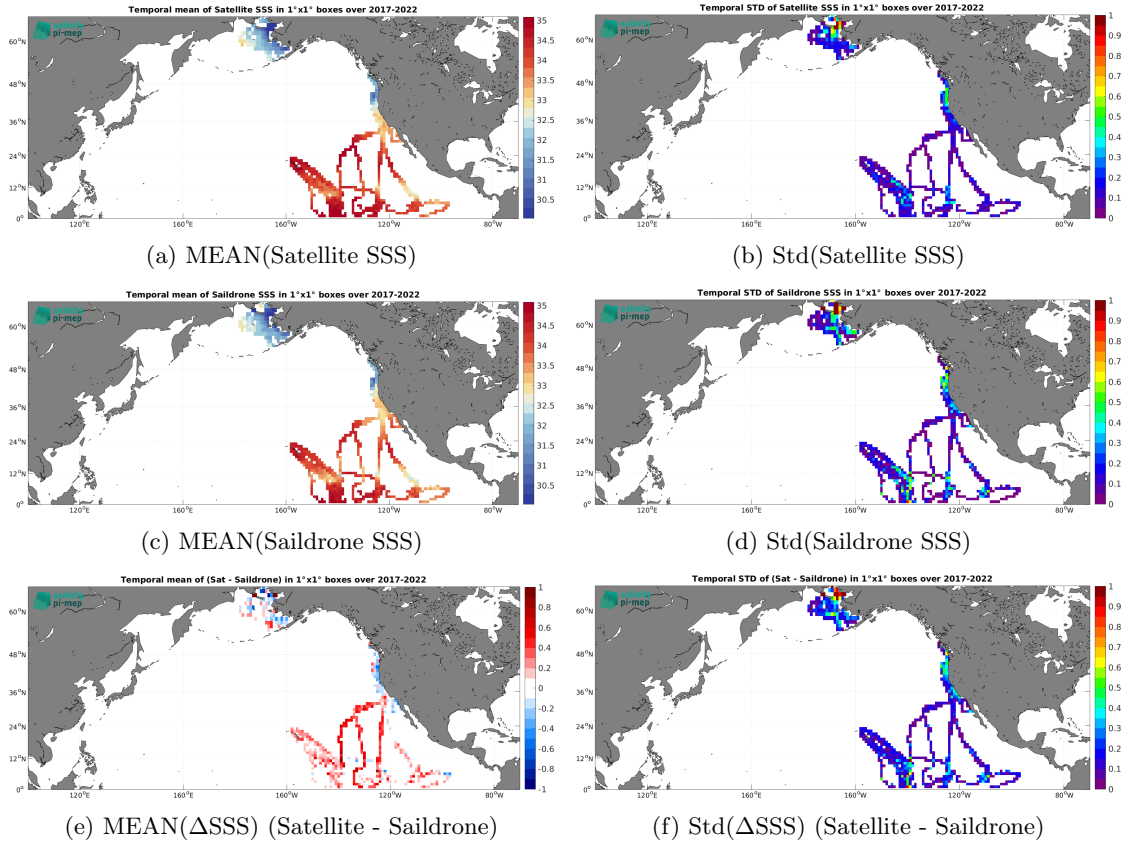
Figure 7: Temporal mean (left) and Std (right) of SSS from CCI SSS L4 Merged-OI v4.41 - 7-day running (ESA) (top), Saildrone (middle), and of \Delta\text{SSS} (Satellite - Saildrone). Only match-up pairs are used to generate these maps.
