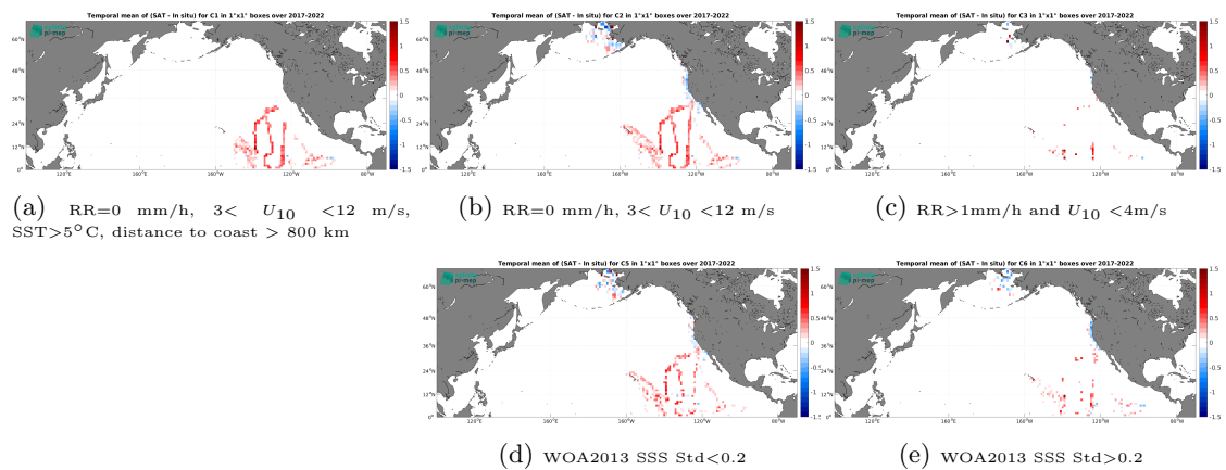
Figure 14: Temporal mean gridded over spatial boxes of size 1^\circ \times 1^\circ of \Delta SSS (CCI SSS L4 Merged-OI v4.41 - 7-day running (ESA) - Saildrone) for 5 different subdatasets corresponding to: RR=0 mm/h, 3 < U_{10} < 12 m/s, SST > 5°C, distance to coast > 800 km (a), RR=0 mm/h, 3 < U_{10} < 12 m/s (b), RR > 1mm/h and U_{10} < 4 m/s (c), WOA2013 SSS Std < 0.2 (d), WOA2013 SSS Std > 0.2 (e).
