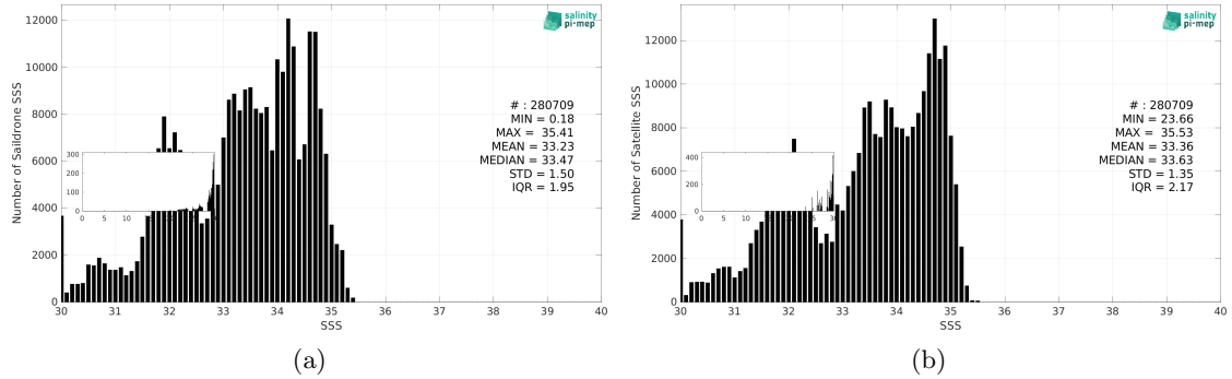
Figure 3: Histograms of SSS from Saildrone (a) and CCI SSS L4 Merged-OI v4.41 - 7-day running (ESA) (b) considering all match-up pairs per bins of 0.1 over the North Pacific Ocean Pi-MEP region and for the full satellite product period.
