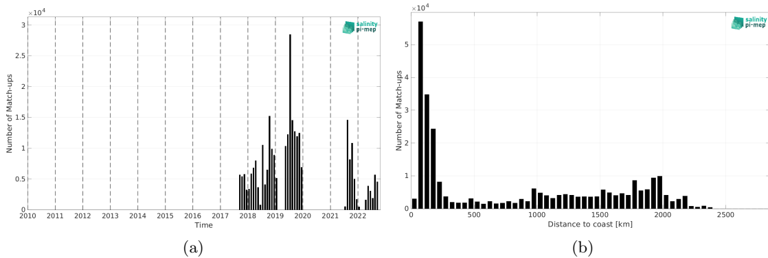
Figure 2: Number of match-ups between Saildrone and CCI SSS L4 Merged-OI v4.41 - 7-day running (ESA) SSS as a function of time (a) and as function of the distance to coast (b) over the North Pacific Ocean Pi-MEP region and for the full satellite product period.
