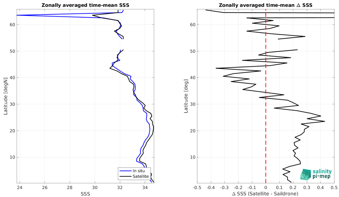
Figure 9: Left panel: Zonal mean SSS from CCI SSS L4 Merged-OI v4.41 - 7-day running (ESA) satellite product (black) and from Saildrone (blue). Right panel: Zonal mean of \Delta SSS (Satellite - Saildrone) for all the collected Pi-MEP match-up pairs estimated over the full satellite product period.
