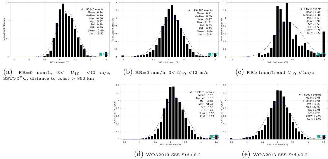
Figure 15: Normalized histogram of \Delta SSS (CCI SSS L4 Merged-OI v4.41 - 7-day running (ESA) - Saildrone) for 5 different subdatasets corresponding to: RR=0 mm/h, 3 < U_{10} < 12 m/s, SST>5°C, distance to coast > 800 km (a), RR=0 mm/h, 3 < U_{10} < 12 m/s (b), RR>1mm/h and U_{10} < 4 m/s (c), WOA2013 SSS Std<0.2 (d), WOA2013 SSS Std>0.2 (e).
