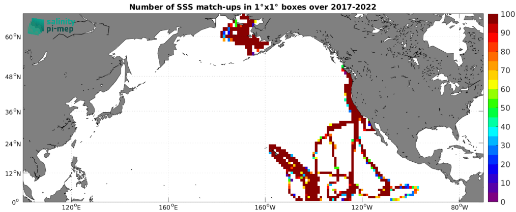
Figure 5: Number of SSS match-ups between Saildrone SSS and the CCI SSS L4 Merged-OI v4.41 - 7-day running (ESA) SSS product for the North Pacific Ocean Pi-MEP region over 1^\circ \times 1^\circ boxes and for the full satellite product period.
