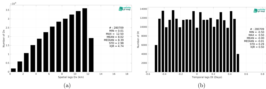
Figure 6: Histograms of the spatial (a) and temporal (b) lags between the location/time of the Saildrone measurement and the date of the corresponding CCI SSS L4 Merged-OI v4.41 - 7-day running (ESA) SSS pixel.
