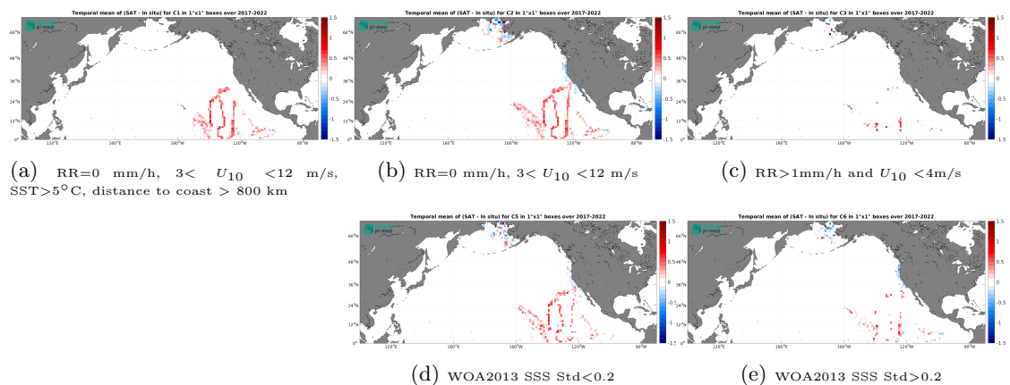
Figure 14: Temporal mean gridded over spatial boxes of size 1^\circ \times 1^\circ of \Delta\text{SSS} (CCI SSS L4 Merged-OI v4.41 - 7-day running (ESA) - Saildrone) for 5 different subdatasets corresponding to: RR=0 mm/h, 3 < U_{10} < 12 m/s, SST > 5°C, distance to coast > 800 km (a), RR=0 mm/h, 3 < U_{10} < 12 m/s (b), RR > 1mm/h and U_{10} < 4 m/s (c), WOA2013 SSS Std < 0.2 (d), WOA2013 SSS Std > 0.2 (e).
